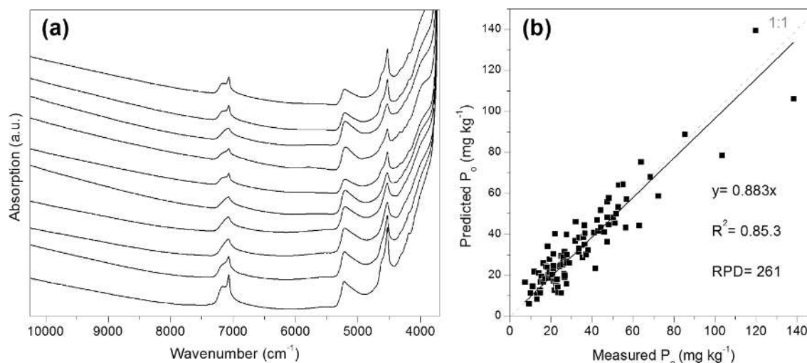
Figure 3: (a) Examples of typical NIR absorption spectra from soil samples (Cambisols). (b) Model calibration results, predicted vs. measured, for NaOH soluble organic P (P o ) (Niederberger et al., 2013, unpublished).
