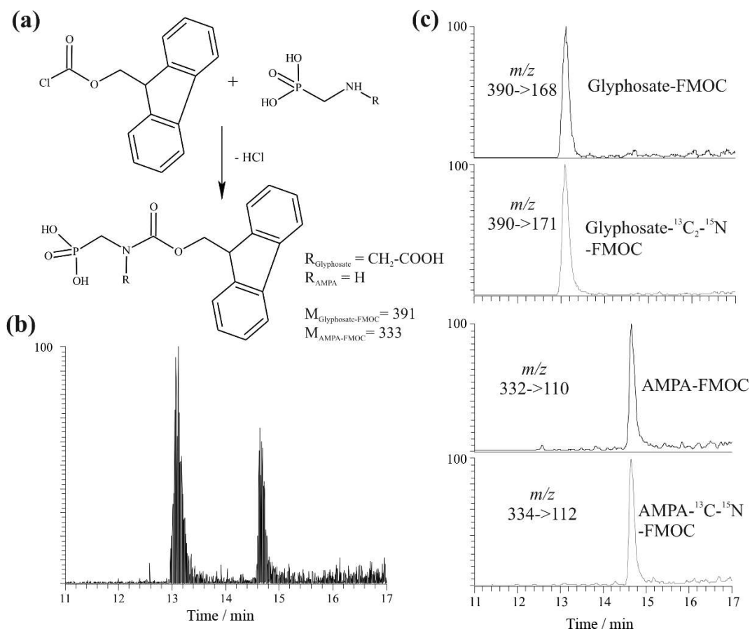
Figure 6: (a) Pre-column derivatization of glyphosate and AMPA: the reaction of FMOCl with glyphosate and AMPA results in the formation of glyphosate-FMOC and AMPA-FMOC with molecular masses of 391 and 333 g mol -1 , respectively. (b) Total Ion Chromatogram of the FMOC-derivatives: the derivatized compounds are separated on a reverse phase liquid chromatography system and detected through Tandem Mass Spectrometry after Electrospray Ionization. (c) Operation in the Selected Reaction Monitoring mode allows detection of the compounds based on the m/z ratios of their product ions. The isotope-labelled glyphosate-1,2- ^{13}\text{C}_2 - ^{15}\text{N} and AMPA- ^{13}\text{C} - ^{15}\text{N} serve as internal standards (Abraham, 2014, unpublished).
