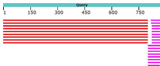
Fig. 2: (A) Sequence of amplified DNA Fragment using BL-1(FP) &BL-1(RP) Nucleotide sequence (863 letters)
