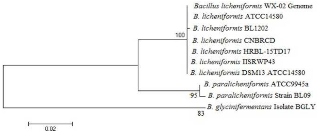
Fig. 5: B. A Tree plot was constructed with the NJ method using 863bp fragment of the Aldo/keto reductase gene showing the relationship of B. licheniformis with other Bacillus spp.
