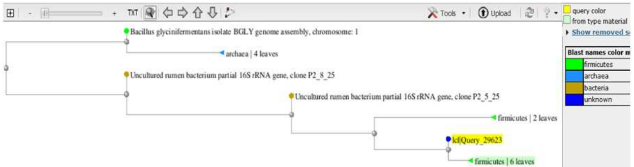
Fig. 5: A. Phylogenetic analysis using query nucleotide sequence
