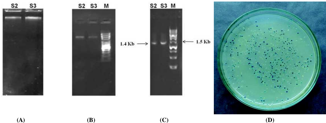
Fig. 1: A-D: (A) Total genomic DNA of representative soil sample S2 containing consortium and genomic DNA S3 of B. licheniformis ; (B) PCR amplification of 16S rDNA region from total genomic DNA of representative soil sample S2 and genomic DNA S3 of B. licheniformis ; (C) PCR amplified product from total genomic DNA by B. licheniformis specific primer of representative soil sample S2 and genomic DNA S3
