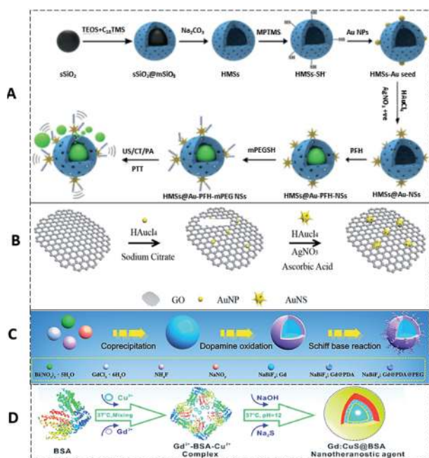
Fig. 8 (A) Schematic illustration of the synthesis of HMSs, HMSs@Au NPs, and HAPPs, 145 reproduced from ref. 145 with permission from the American Chemical Society, copyright 2017. (B) rGO/Au NPs nano-composite, 147 reproduced from ref. 147 with permission from the American Chemical Society, copyright 2019. (C) NaBiF 4 :Gd-PDA-PEG NPs, 150 reproduced from ref. 150 with permission from the American Chemical Society, copyright 2020. (D) Gd:CuS@BSA NPs, 151 reproduced from ref. 151 with permission from the American Chemical Society, copyright 2016.
