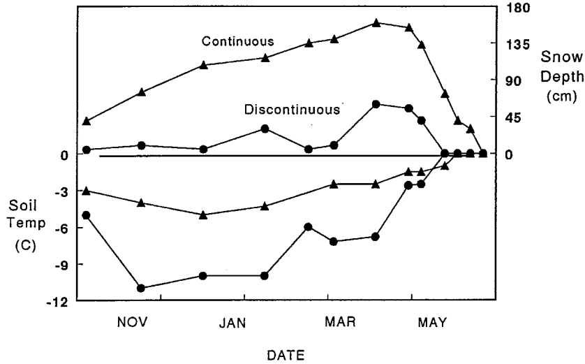
Figure 1. Snow depth (top) and soil surface temperature (bottom) under shallow, discontinuous and deep, continuous snowpacks, 1994. ( n = 3 , SE is smaller than size of symbol).
