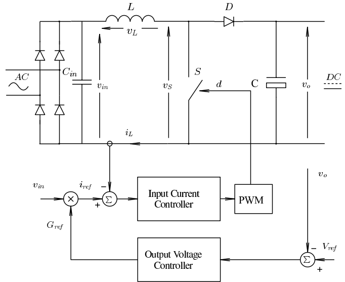
Fig. 1. The boost PFC converter, together with its control loops.
