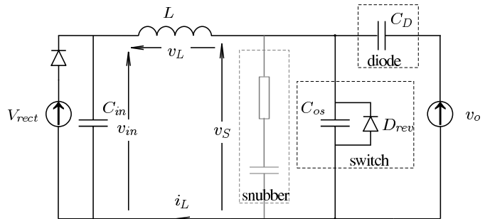
Fig. 2. Black: Equivalent network for the boost converter when both diode D and switch S are blocked; Gray: snubber
