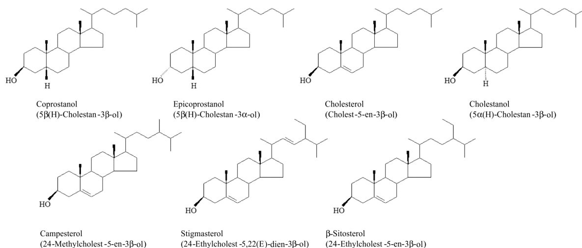
Figure 2. Chemical structures of the analyzed sterols and ketone.
