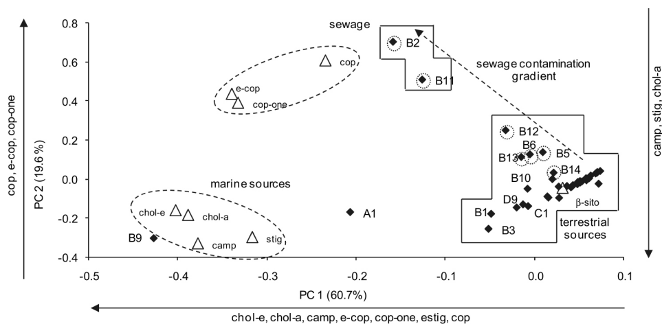
Figure 4. Principal component analysis between analyzed sterols for the sediments collected on the Paranaguá Bay. The steroid abbreviations means: cop (coprostanol), e-cop: (epicoprostanol), cop-one (coprostanone), chol-e (cholesterol), chol-a (cholestanol), camp (campesterol), stig (stigmasterol) and \beta -sit ( \beta -sitosterol).
