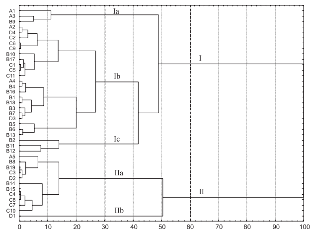
Figure 5. Cluster analyses according to general sources (fecal, terrestrial or marine sources) in the total sterols for the sediments in the Paranaguá Estuarine System. I and II represent subgroups explained in the text.
