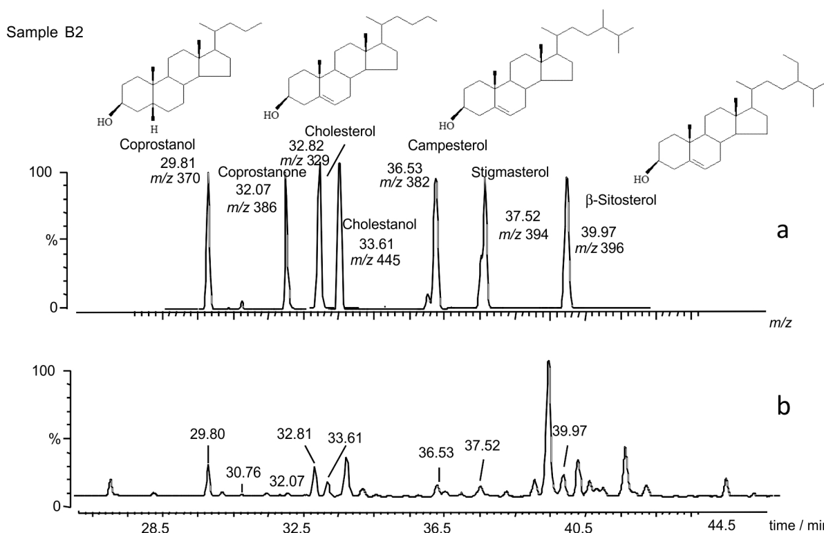
Figure 3. Example of (a) mass and (b) total ion chromatograms of steroids in representative surface sediment sampling site B2 in the Paranaguá Estuarine System.
