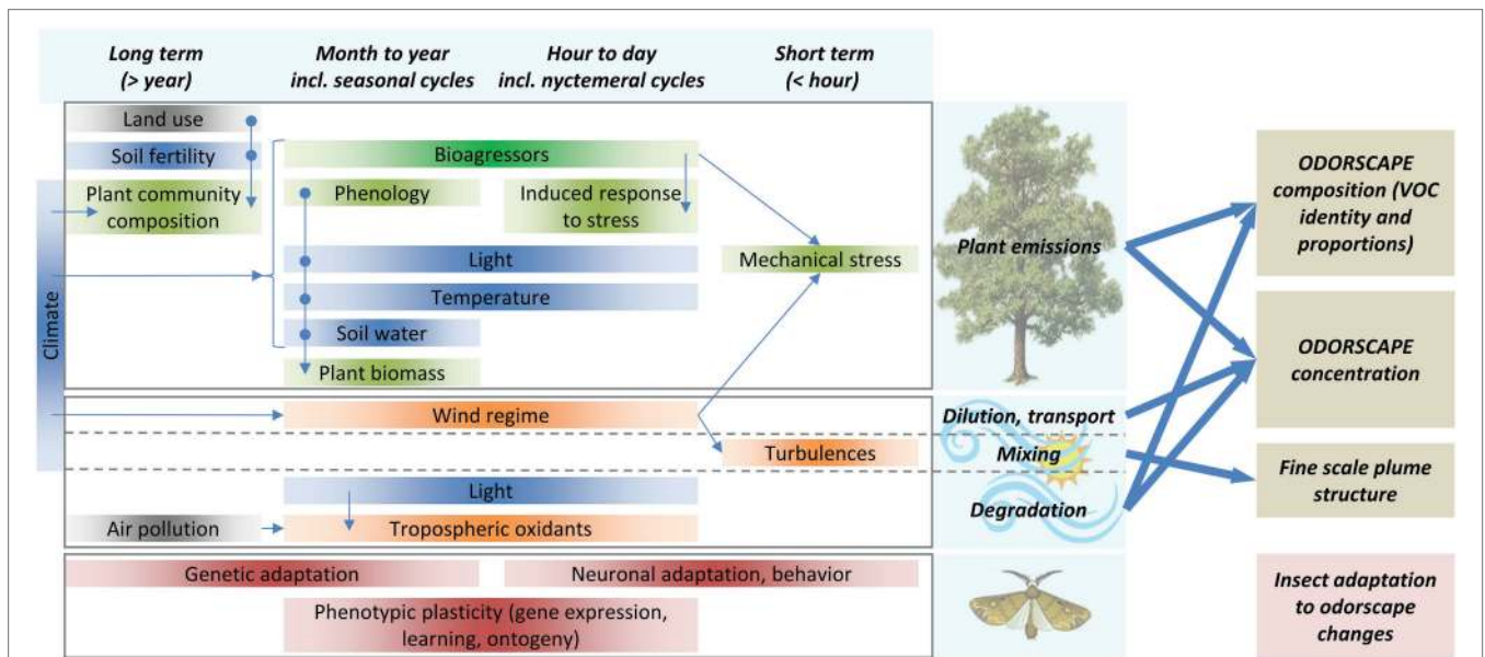
FIGURE 2 | Odorscapes are highly variable at a diversity of time scales. The left part of this chart depicts the factors that determine volatile emissions by plants (top), atmospheric processes (middle), and the processes by which insects can adapt to changes in their olfactory environment (bottom), classified horizontally by the time scale at which they act or vary. Thin arrows depict indirect impacts, through influence on another factor. Box color: dark blue = climate and soil factors, green = plant physiology and ecology, orange = atmospheric physico-chemistry, brown = insect adaptation processes, gray = anthropic factors. Although this is not represented for readability issues, extremes of most climate and soil factors do cause stress responses in plants. VOC sources other than plants (especially anthropogenic VOC) are ignored. On the right side, thick arrows depict how plant emissions and atmospheric processes determine the characteristics of the odorscape.
