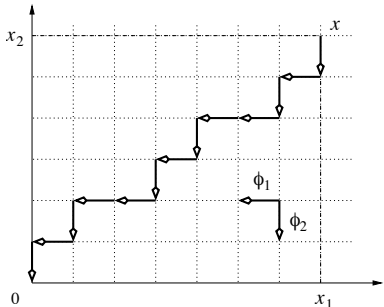
Figure 1: The balance function \Phi(x) is equal to the weight of any direct path from state x to state 0.
