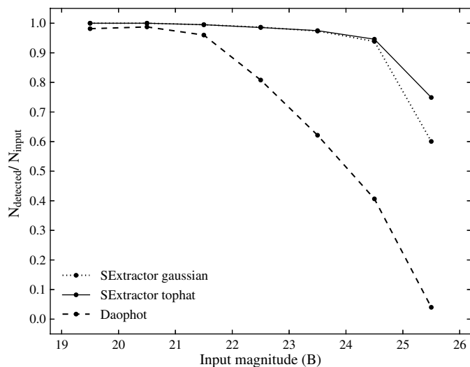
FIG. 2.—Ratio between detected and input sources for different magnitude bins. The dotted and the solid lines refer to SExtractor used with a Gaussian and a top-hat filter, respectively, while the dashed line refers to values obtained with DAOPHOT.
