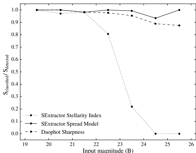
FIG. 6.—Ratio between stars classified by Stellarity Index ( dotted line ) and Spread Model ( solid line ) from SExtractor with threshold values respectively to 0.98 and 0.005, and by DAOPHOT sharpness ( dashed line ) with a threshold value equal to zero and detected stars, as function of input magnitude.
