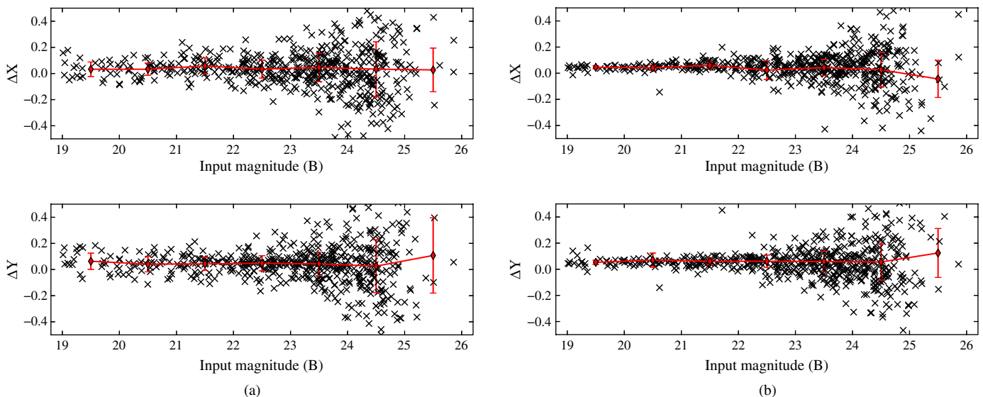
FIG. 8.—Difference between barycenter coordinates estimated by DAOPHOT ( left ) and by SExtractor ( right ), and input coordinates and as a function of input magnitude for detected stars. Superimposed red points and solid red lines draw the mean and standard deviation values reported in top part of Table 5. See the online edition of the PASP for a color version of this figure.
