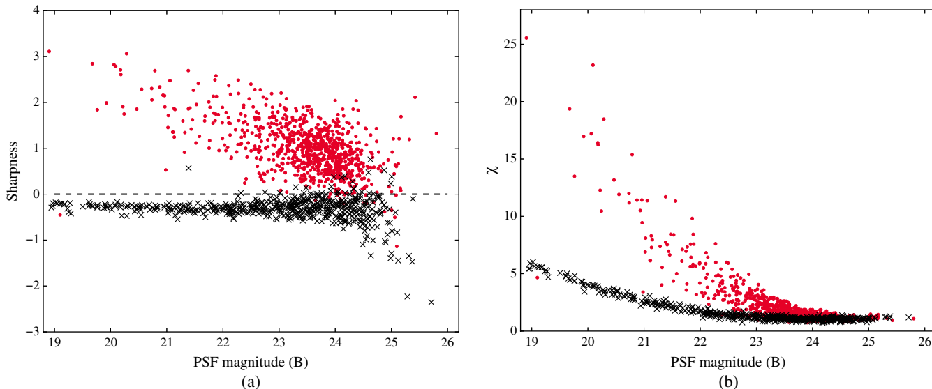
FIG. 4.—Distribution of DAOPHOT sharpness ( left panel ) and \chi ( right panel ) as a function of the PSF magnitude for simulated stars ( diagonal crosses ) and galaxies ( points ). In the left panel the dashed line at zero sharpness is the adopted separation limit for the star/galaxy classification (see § 5.2). See the online edition of the PASP for a color version of this figure.
