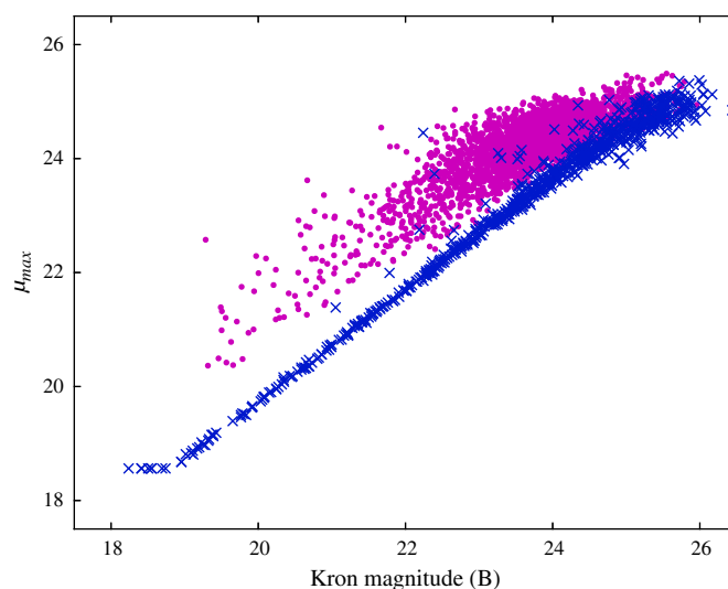
FIG. 1.— \mu_{\max} as a function of the Kron magnitude for stars (diagonal crosses) and galaxies (points) in the SExtractor catalog. See the online edition of the PASP for a color version of this figure.
