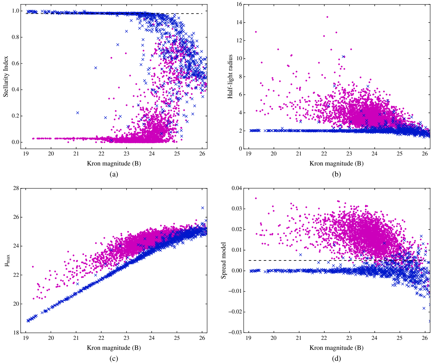
FIG. 5.—Distribution of SEExtractor stellarity index (a), half-light radius (b), \mu_{\max} (c) and spread model (d), as a function of the Kron magnitudes for simulated stars (diagonal crosses) and galaxies (points). The dashed line in (a) and (d) is the adopted separation limit for the star/galaxy classification (see § 5.2). See the online edition of the PASP for a color version of this figure.
