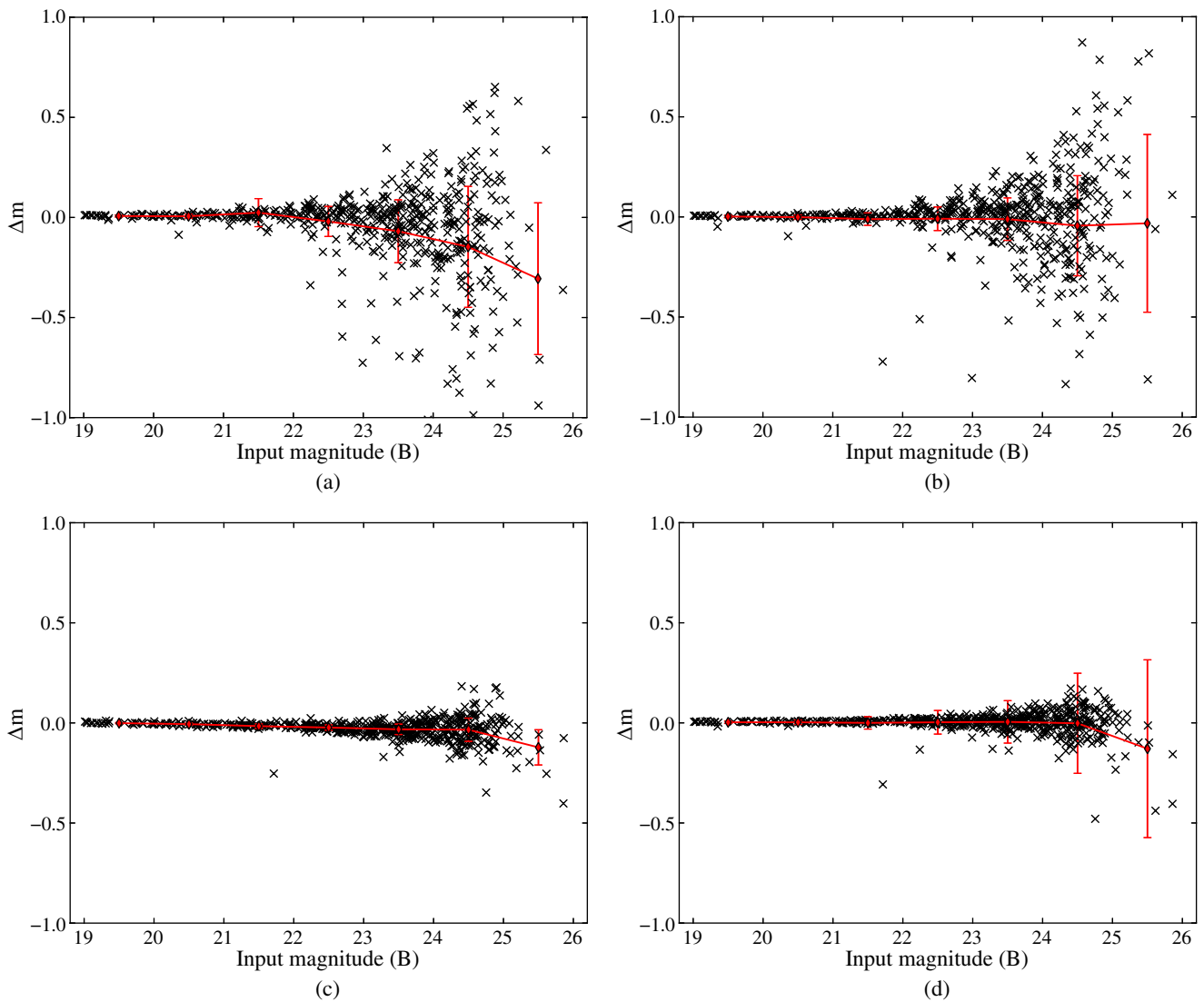
FIG. 7.— Top : Residuals between aperture magnitudes estimated by DAOPHOT ( left ) and by SExtractor ( right ), and input magnitudes for detected stars. Bottom : Residuals between PSF magnitude estimated by DAOPHOT ( left ) and by SExtractor ( right ), and input magnitude for detected stars. Superimposed red points and solid red lines draw the mean and standard deviation values reported in Table 3. See the online edition of the PASP for a color version of this figure.
