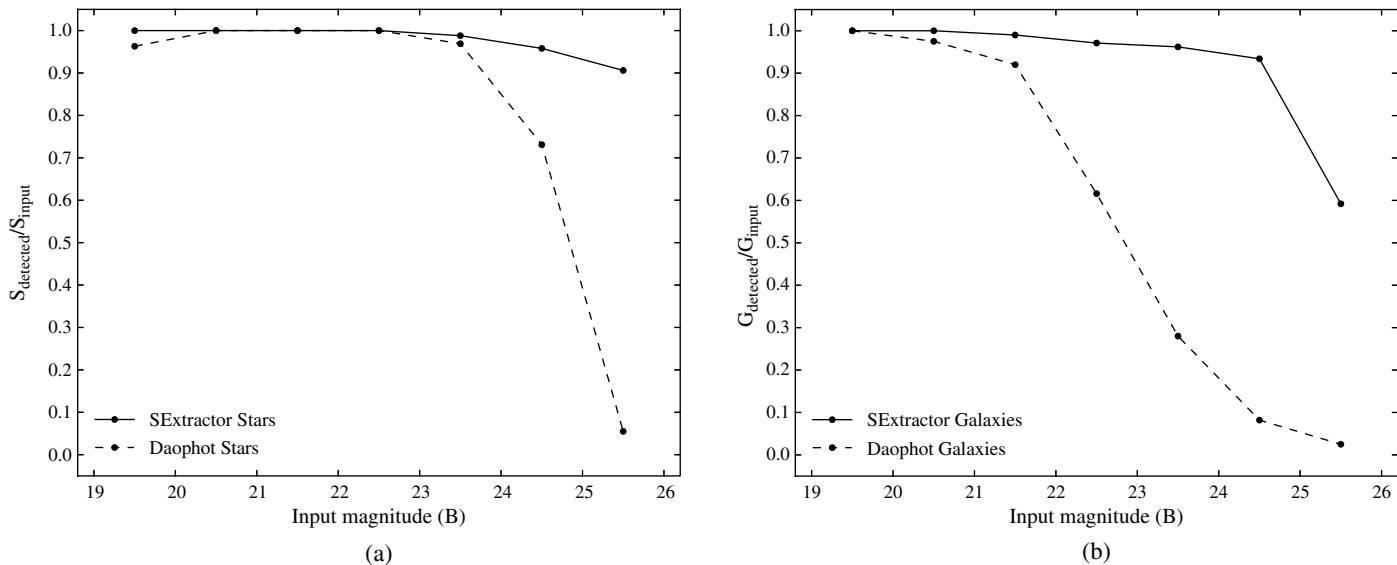
FIG. 3.—The left panel shows the ratio between the numbers of detected and input stars as a function of magnitude bins, as obtained by SExtractor ( solid line ) and by DAOPHOT ( dashed line ); in the right panel are plotted the same quantities, but for galaxies.
