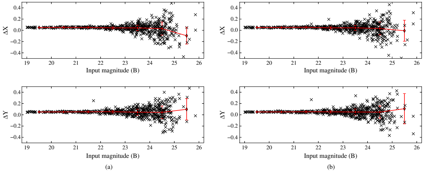
FIG. 9.—Difference between PSF-corrected and input coordinates estimated by DAOPHOT ( left ) and by SExtractor ( right ), as a function of input magnitude for detected stars. Superimposed red points and solid red lines draw the mean and standard deviation values reported in bottom part of Table 5. See the online edition of the PASP for a color version of this figure.
