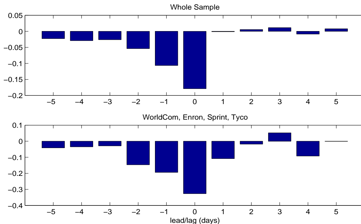
Figure 1: Cross Correlation of Stock Returns and CDS Changes.
