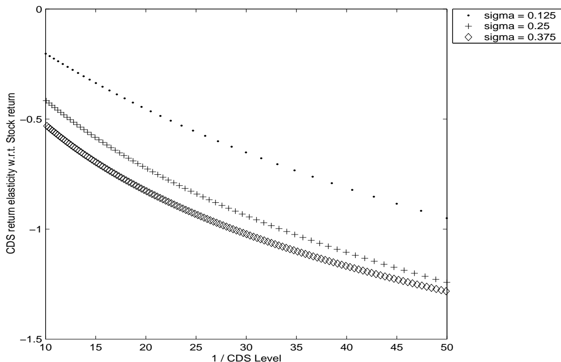
Figure 2: Merton (1973) model credit-spread elasticity.
