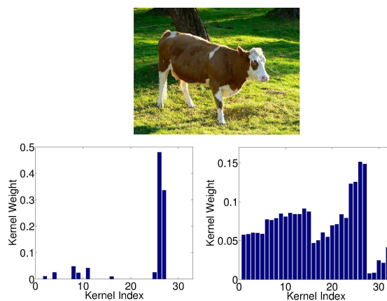
Figure 4. Images of a typical highly ranked cow image and kernel weights from l_1 -MKL (left) and l_{1.333} -MKL (right).
