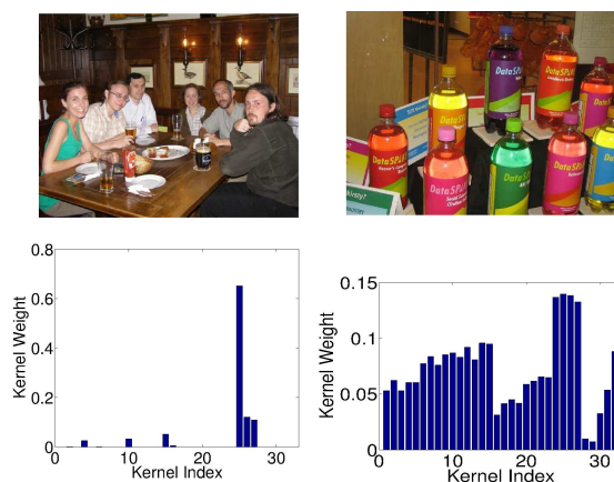
Figure 3. Images of typical highly ranked bottle images and kernel weights from l_1 -MKL (left) and l_{1.333} -MKL (right).
