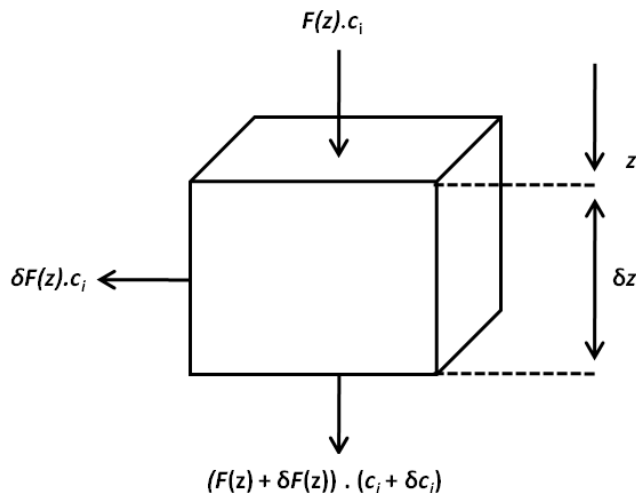
Figure A1. Schematic overview of solute mass balance where F is the rate of percolation ( \text{myr}^{-1} ) at depth z and c is the concentration of ion i in solution ( \text{gm}^{-3} ). Adapted from Kirkby (1985).
