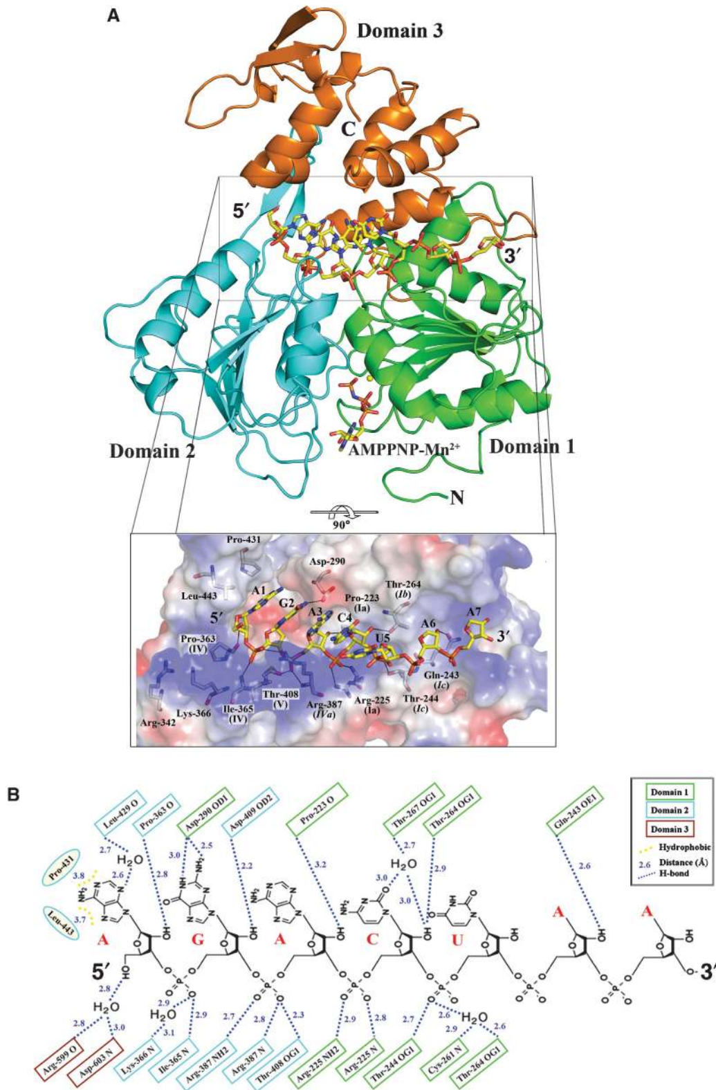
Figure 1 The flavivirus NS3h-RNA-AMPPNP ternary complex. (A) Cartoon representation of NS3h bound to ssRNA and AMPPNP, a non-hydrolysable ATP analogue shown as sticks. The Rec-A-like subdomains 1 and 2 are coloured in green and cyan, respectively. The manganese ion is represented as a yellow sphere. Inset: magnified view of the interactions between the protein and its RNA ligand, using a colour-coded representation of the NS3h electrostatic surface potential. The colour scale is -10 kT (red) to +10 kT (blue). Residues that contact RNA are displayed as sticks and labelled. Also indicated their motif (see also Figure 5). Domain 3 was omitted for clarity. (B) Schematic representation of the interactions observed between NS3h and ssRNA (RNA 12 ). Notice several contacts established with the 2'-hydroxyl groups of the ribose moieties.
