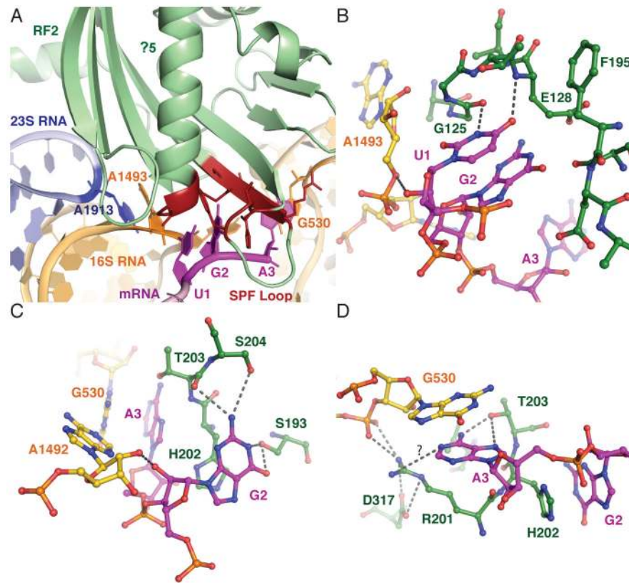
Fig. 2. Interaction of RF2 with the stop codon in the decoding center. A. Overview of the decoding center showing the UGA stop codon (magenta). Domain 2 of RF2 is shown in green, except for parts interacting with the codon, which are shown in red. Key bases from 16S RNA and A1913 of 23S RNA are also shown. (B to D). Details of interactions at the first (B), second (C) and third (D) positions of the stop codon with elements of RF2 and the decoding center.
