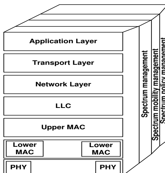
Figure 3. Cognitive Radio Architecture
