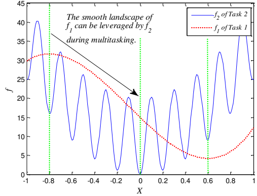
Fig. 5. A simple task can be exploited by a complex task in the same multitasking environment for faster convergence.
