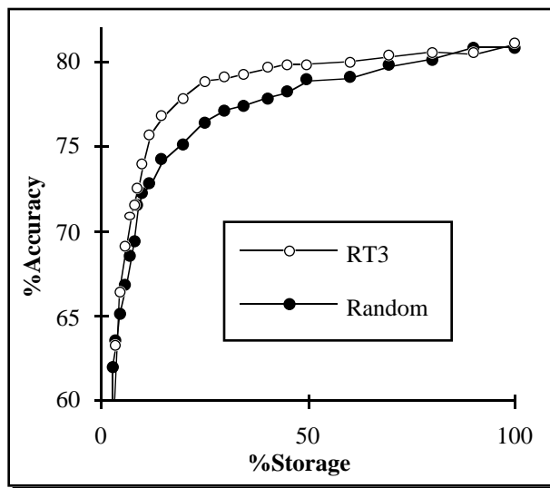
Figure 2: Generalization Accuracy for RT3 vs. Randomly removing instances.
