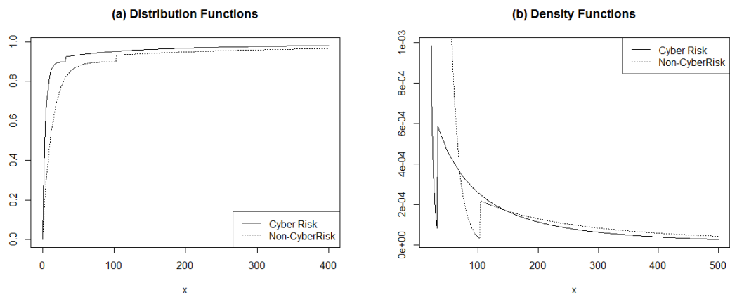
Figure C2 Estimated distribution and density function
