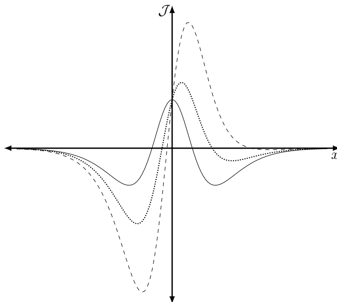
Figure 1. The form of \mathcal{J} in (4.63) is plotted for generic fixed values of c_{\mathcal{P}}, c_{\mathcal{J}}, a, v and for different values of \eta_1 . Note that when the integration constant \eta_1 vanishes, \mathcal{J} becomes an even function of x (solid line).
