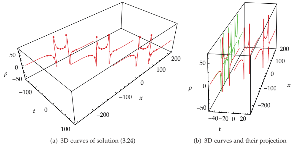
Figure 7: Evolvement graphs of 3D-curves along with the time and their projection curve.
