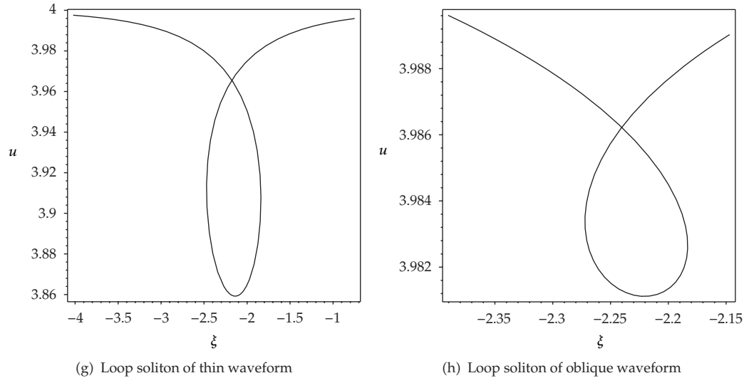
Figure 1: The profiles of multiwaveform of (3.6) for the given parameters and different \varepsilon -values: (a) \varepsilon = 1.2 ; (b) \varepsilon = 1.26 ; (c) \varepsilon = 1.4 ; (d) \varepsilon = 1.99 ; (e) \varepsilon = 2 ; (f) \varepsilon = 2.2 ; (g) \varepsilon = 3 ; (h) \varepsilon = 5 .
