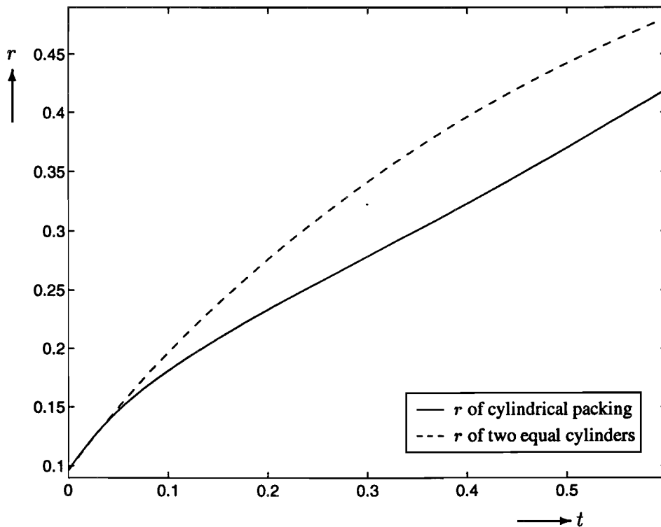
Figure 6: The contact radius r development of the cylindrical packing compared with the exact analytical solution of the coalescence of two equal cylinders shows only an agreement during the early stage. At later time stages the neck radius of the cylindrical packing develops much slower.
