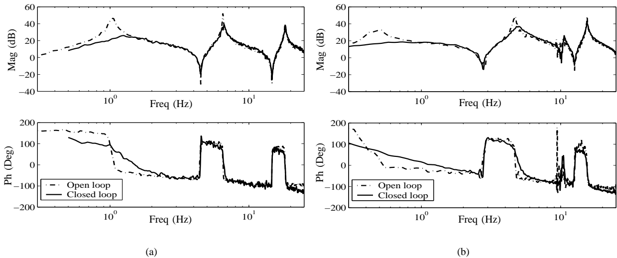
Fig. 6. Magnitude response of G_m(s)G_2(s) (---) and the closed loop system between coupling torque and tip angle reference (—), (a) M_P = 0.0 kg and (b) M_P = 0.3 kg. Note that in both the cases, there is substantial damping in the first two resonant modes.
