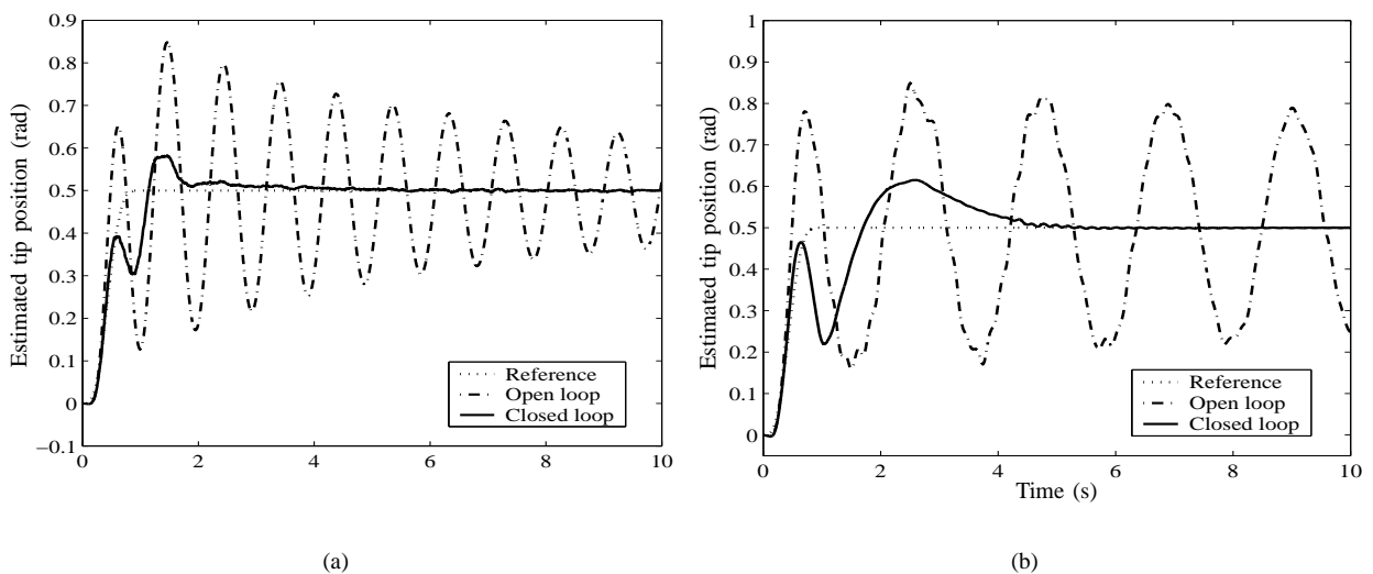
Fig. 9. Time response of the estimated tip angle obtained from experimental data, (a) M_P = 0.0\text{kg} and (b) M_P = 0.3\text{kg} . Reference (...) and estimated tip position in open loop (---) and closed loop (—)
