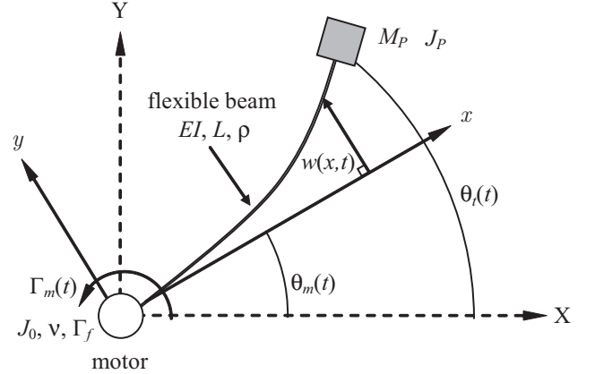
Fig. 2. Parametric representation of the flexible arm system
