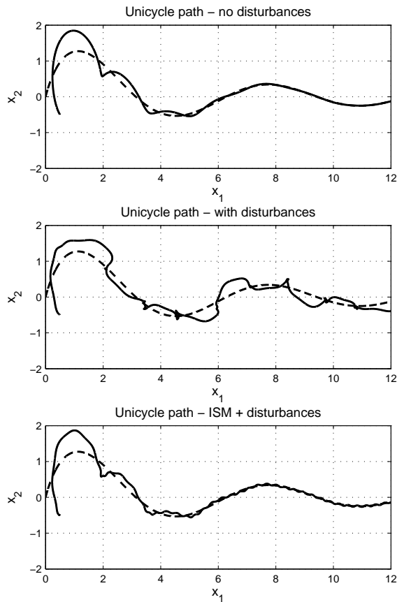
Fig. 1. The path of the unicycle in case of high level controller with no disturbances (top), high level controller with disturbances (middle) and high level controller plus ISM with disturbances (bottom). The reference trajectory is depicted as a dashed line, while the actual ones are represented as solid lines
