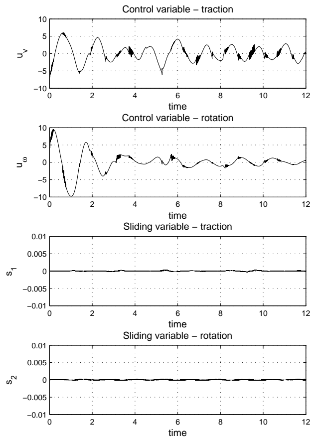
Fig. 2. Time evolution of (from top to bottom) of the control variables and the components of the sliding manifold, for the simulation example regarding the use of high level controller and ISM with disturbances
