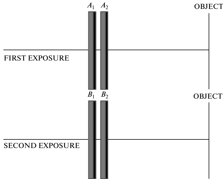
Fig. 2. Sandwich holography.
