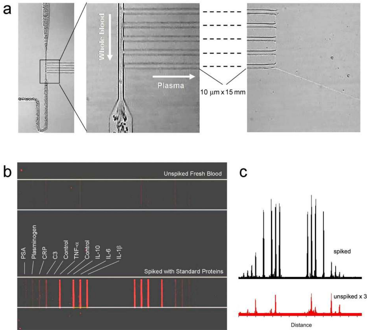
Figure 4. IBBC for the rapid measurement of a panel of serum biomarkers from a finger-prick of whole blood. (a) Optical micrographs showing the effective separation of plasma from fresh whole blood. A few red blood cells were occasionally seen downstream of the plasma channels, but this did not
