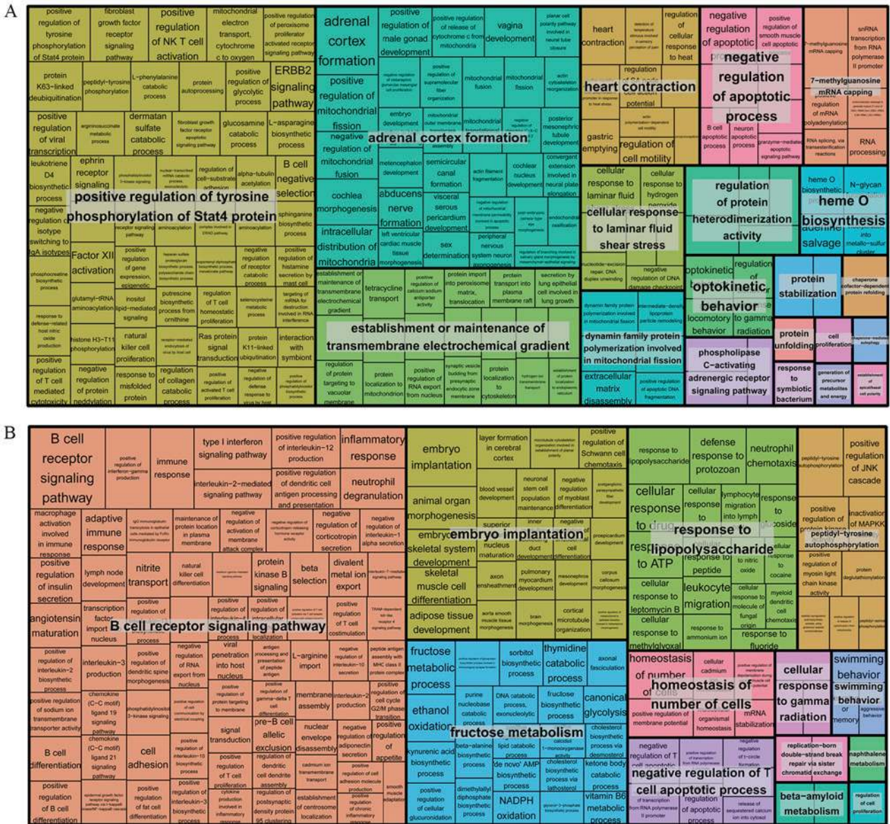
Figure 5. Over representation of enriched biological processes for DEGs. (A) REVIGO gene ontology treemap for upregulated DEGs by meta-analysis. (B) REVIGO gene ontology treemap for downregulated DEGs by meta-analysis. DEGs, DEGs, differentially expressed genes.
