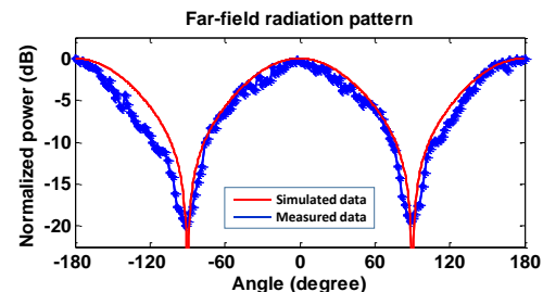
Figure 5. Measured far field radiation pattern (blue) of the bowtie antenna at a frequency of 10.5GHz. Simulated radiation pattern is also overlaid (red).
