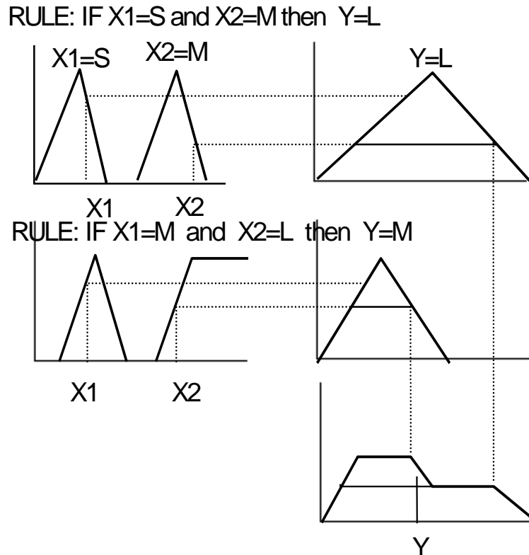
Figure 2: Fuzzy inference
