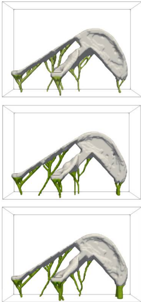
Figure 9 Topology optimized component (white) and support layouts (green) for the application case, with machining accuracy u_{\max} set to 100 (top), 10 and 1.0 \mu\text{m}
