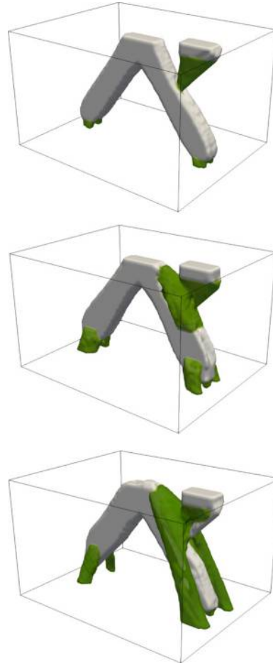
Figure 6 Topology optimized component (white) and support layouts (green) for the test problem, with machining accuracy u_{max} set to 25 \mu\text{m} (top), 10 \mu\text{m} and 2.5 \mu\text{m} .
