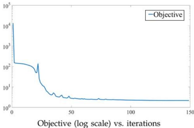
Figure 12 Convergence history of the u_{\max} = 10 \mu\text{m} application case
