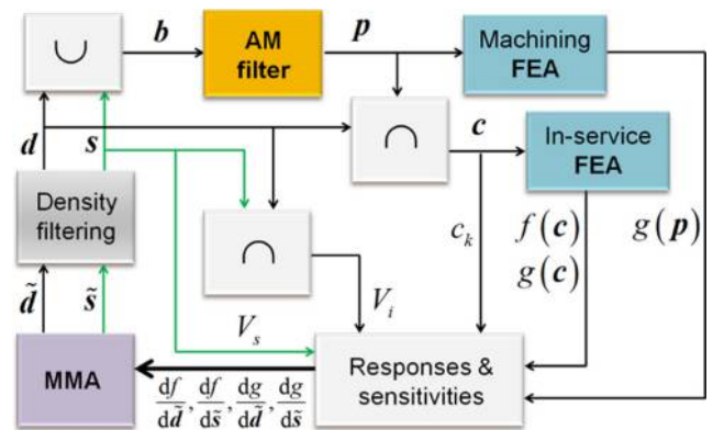
Figure 4 Graphical representation of the optimization process
