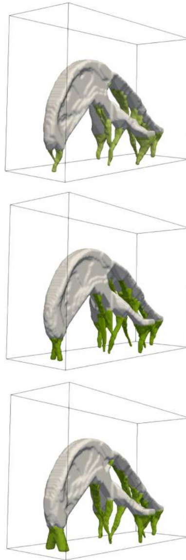
Figure 10 Topology optimized component (white) and support layouts (green) for the application case, with machining accuracy u_{\max} set to 100 (top), 10 and 1.0 \mu\text{m}
