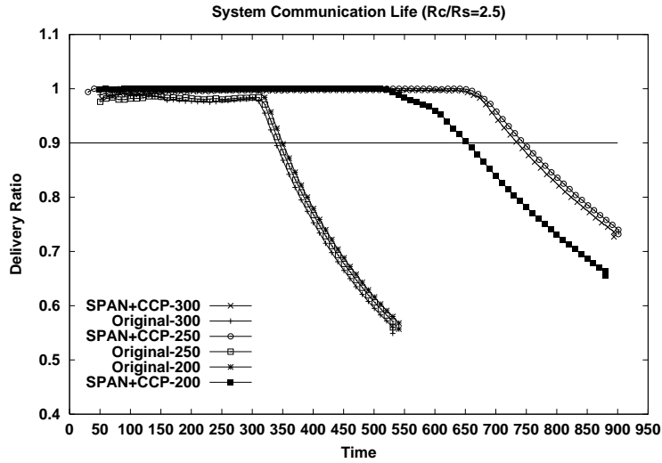
Figure 13. System Communication Life Time
