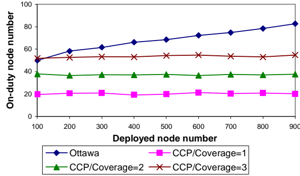
Figure 7. Comparison of active node number
