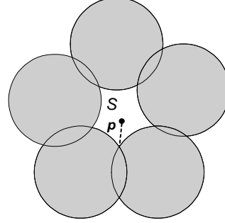
Figure 2. A Coverage Patch Bounded by Sensor Arcs
