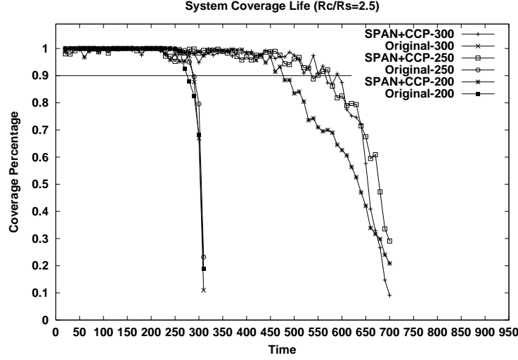
Figure 14. System Coverage Life Time
