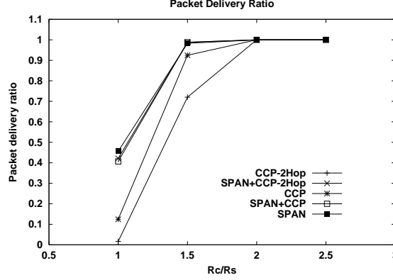
Figure 11. Packet Delivery Ratio vs. R_c/R_s
