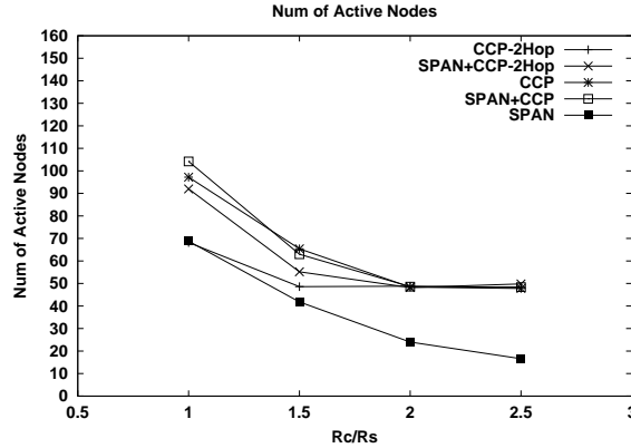
Figure 12. Number of active nodes vs. R_c/R_s
