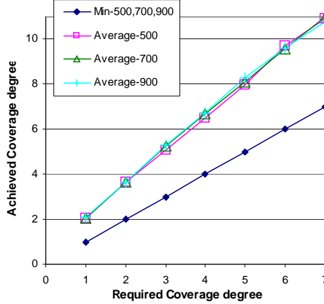
Figure 8. Coverage degree vs. Required Coverage Degree
