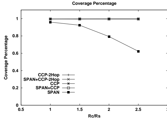
Figure 10. Coverage Degree vs. R_c/R_s
