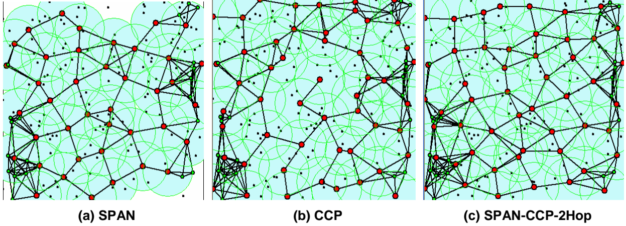
Figure 9. Network Topology and Coverage in a Typical Run ( R_c/R_s = 1.5 )
