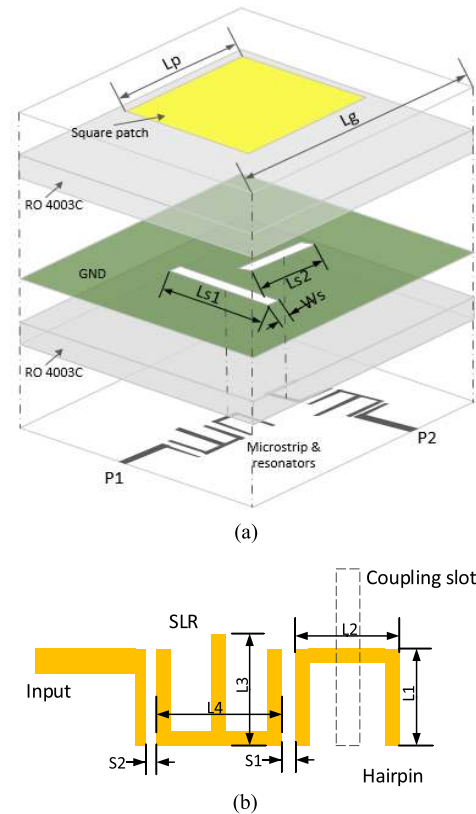
FIGURE 5. Configuration of the proposed low frequency-ratio DBDP filtering antenna (Antenna-I): (a) exploded view; (b) feeding resonators of each polarization. L_p = 17.8 mm, L_g = 50 mm, L_{s1} = 11.8 mm, L_{s2} = 10.3 mm, W_s = 0.9 mm, L_1 = 5.8 mm, L_2 = 4 mm, L_3 = 7 mm, L_4 = 6.5 mm, S_1 = 1.2 mm, S_2 = 0.3 mm.
