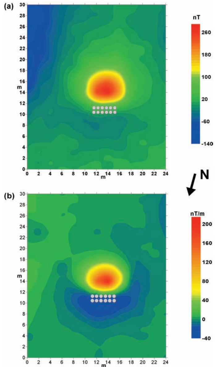
Figure 2. Magnetic anomaly maps of the total intensity field (a) and the vertical magnetic gradient (b).
