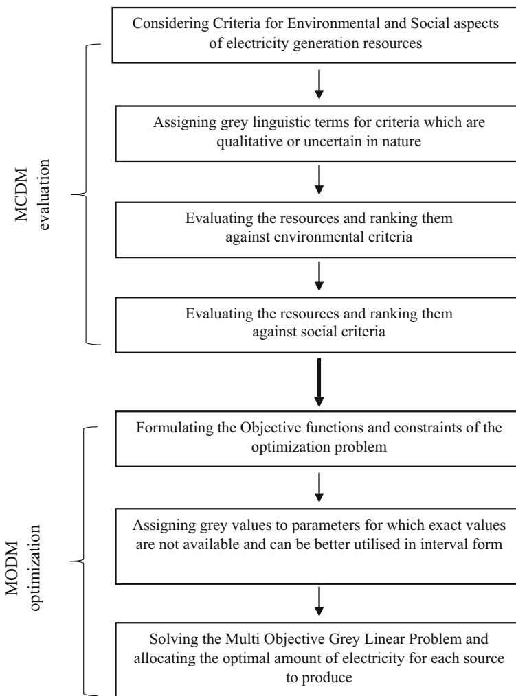
Fig. 1 Solution procedure of GRA–MOGLP integrated approach
