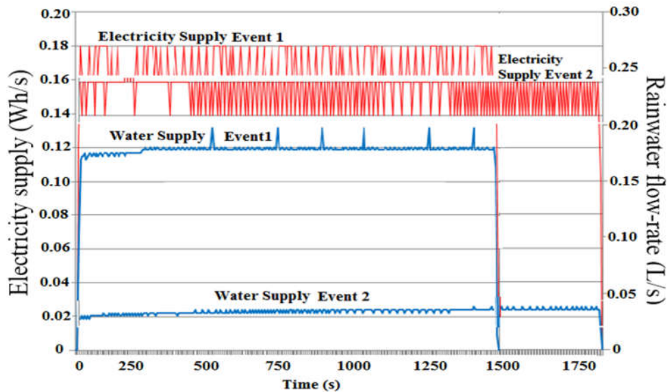
(a) Pump performance comparison from two irrigation events taken from the same system
