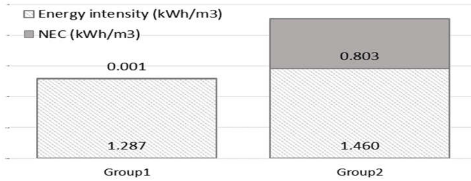
(c) Pump NEC and total energy intensity (kWh/m³)
