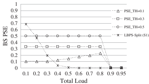
Figure 16. Base station (BS) power-saving efficiency ( PSE ) of load-based power saving (LBPS)-split: strategy 1 versus strategy 2.
