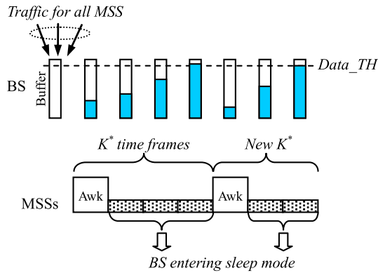
Figure 1. Base station (BS) power saving in load-based power saving-aggr under strategy 1. MSS, mobile subscriber station.
