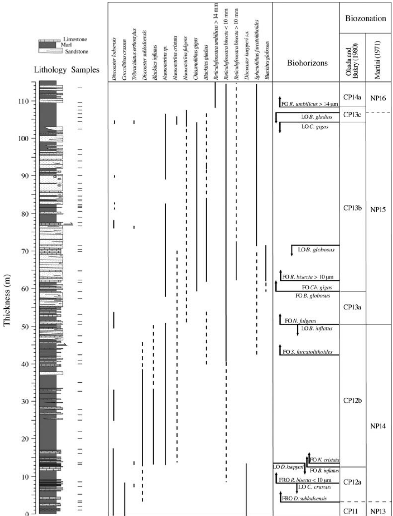
Fig. 5. Stratigraphic distribution of relevant calcareous nannofossils and biozonation of the Agost section. Dashed lines indicate discontinuous occurrences. The position of the studied samples is plotted against the stratigraphic log of the section.
