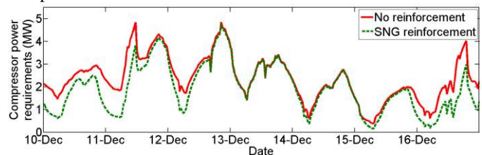
Fig. 10. Power consumption of compressors E and F (Fig. 2(b)) for different cases.
