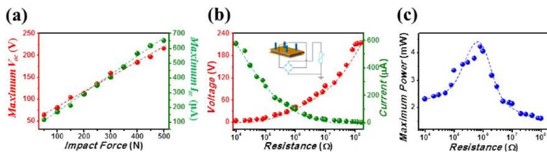
Figure 4. (a) Dependence of the I_{sc} and V_{oc} on the contact force. Larger contact force corresponds to higher current and voltage. The points represent peak value of electric signals while the lines are the fitted results. (b) Dependence of the output current on external load resistance under contact force applied by a human palm. Increased load resistance results in lower output current but higher output voltage. The points represent peak values of electric signals while the curves are fitted result. (c) Dependence of the output power on external load resistance under contact force applied by a human palm, indicating maximum output power when R = 1.0 M \Omega . The curve is a fitted line.
