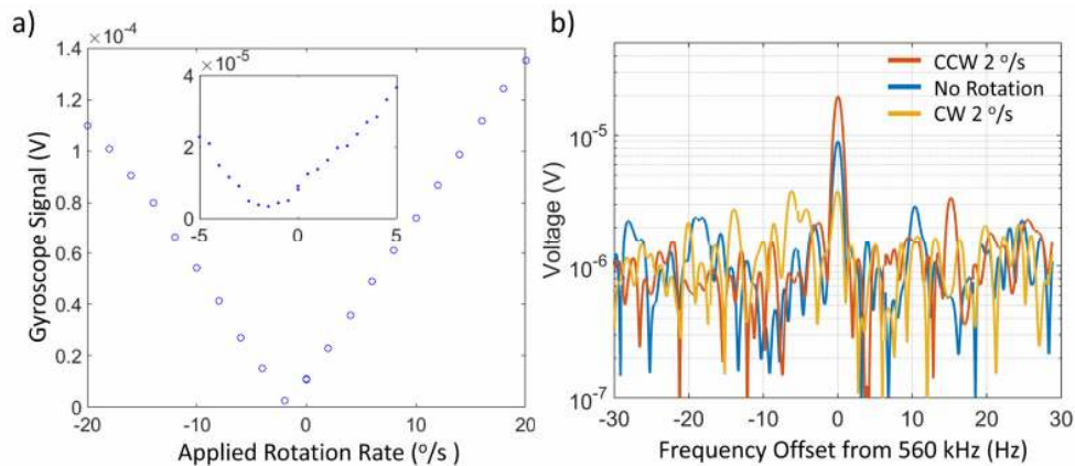
Fig. 16. (a) IOD driven gyroscope's signal versus the rotation rate. Inset shows a zoom-in of small range of the rotation rate. (b) The spectra on the ESA of CW and CCW 2^\circ/\text{s} and zero-rotation. The plot is centered at the 560 kHz modulation frequency with the resolution width of 1 Hz.
