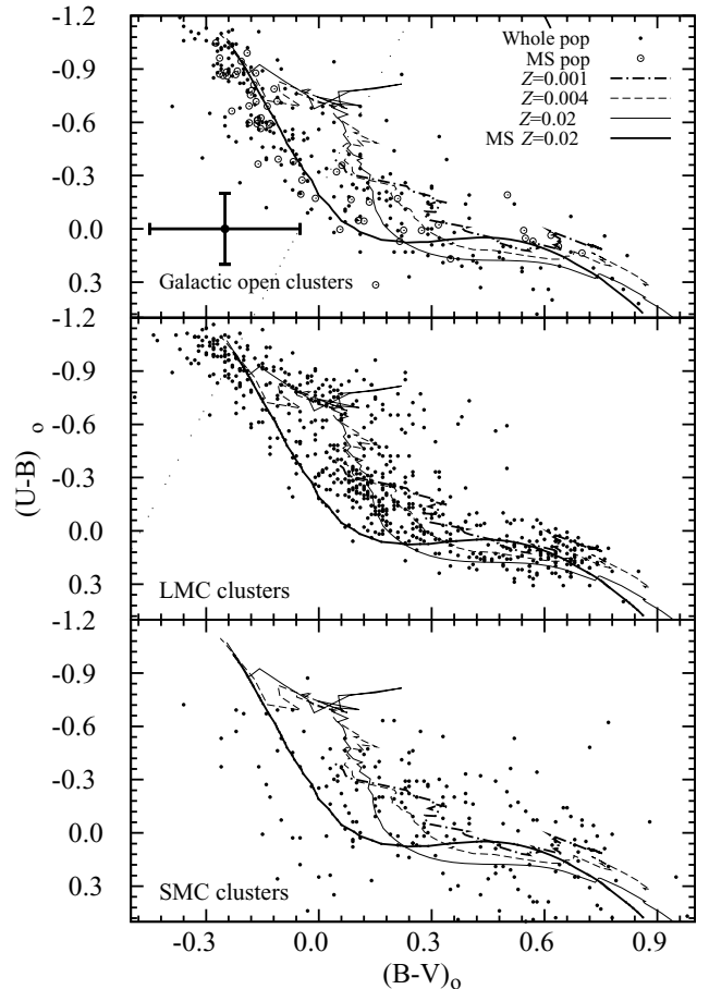
Figure 20. ( U - B ) 0 versus ( B - V ) 0 synthetic colour–colour diagram compared with the observational data of Galactic open clusters (whole population: Pandey et al. 1989; Lata et al. 2002, MS population: present work), LMC (Bica et al. 1996) and SMC (RZ05) clusters.
