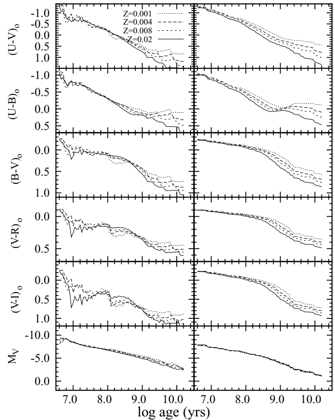
Figure 5. Left-hand panel: effect of metallicity on the integrated magnitude and colours of synthetic clusters (whole population) having a Salpeter mass function and Z = 0.004, 0.008, 0.02 . Right-hand panel: same as left-hand panel, but for the MS population.
