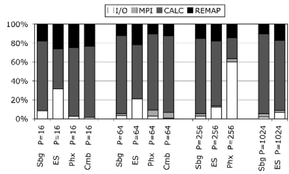
Figure 6. Relative timings for W (16 gangs)
