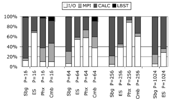
Figure 2. Relative timings for MADbench
