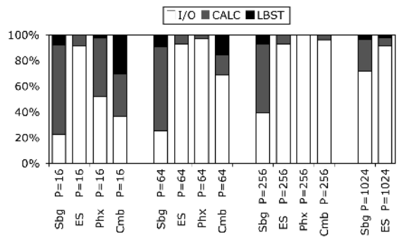
Figure 3. Relative timings for dSdC
