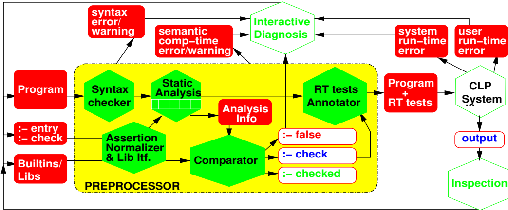
Fig. 2. Architecture of the Preprocessor
