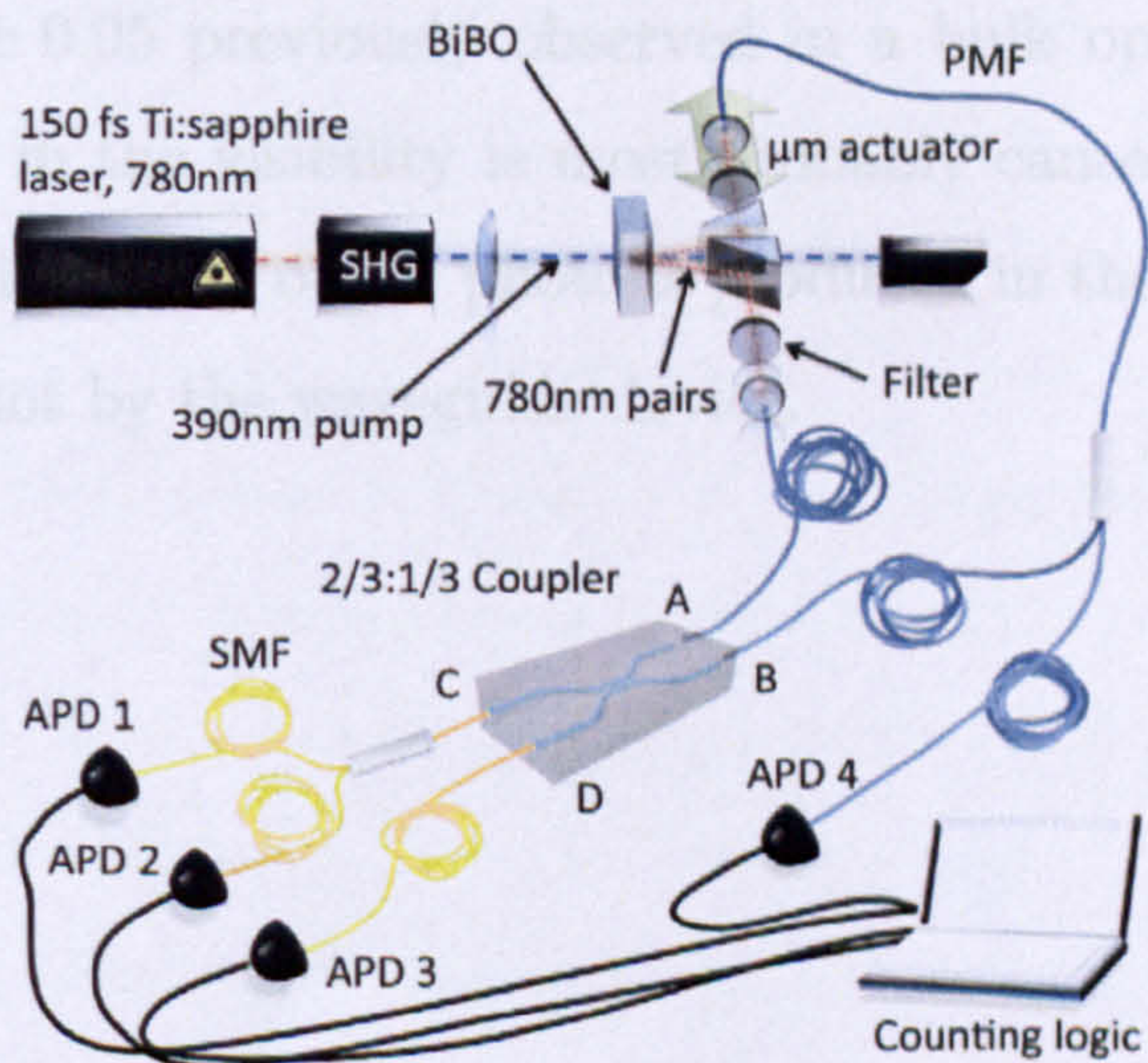
Figure 5.6: Schematic representation of the experimental setup to measure the 3-photon generalized non-classical interference dip.
