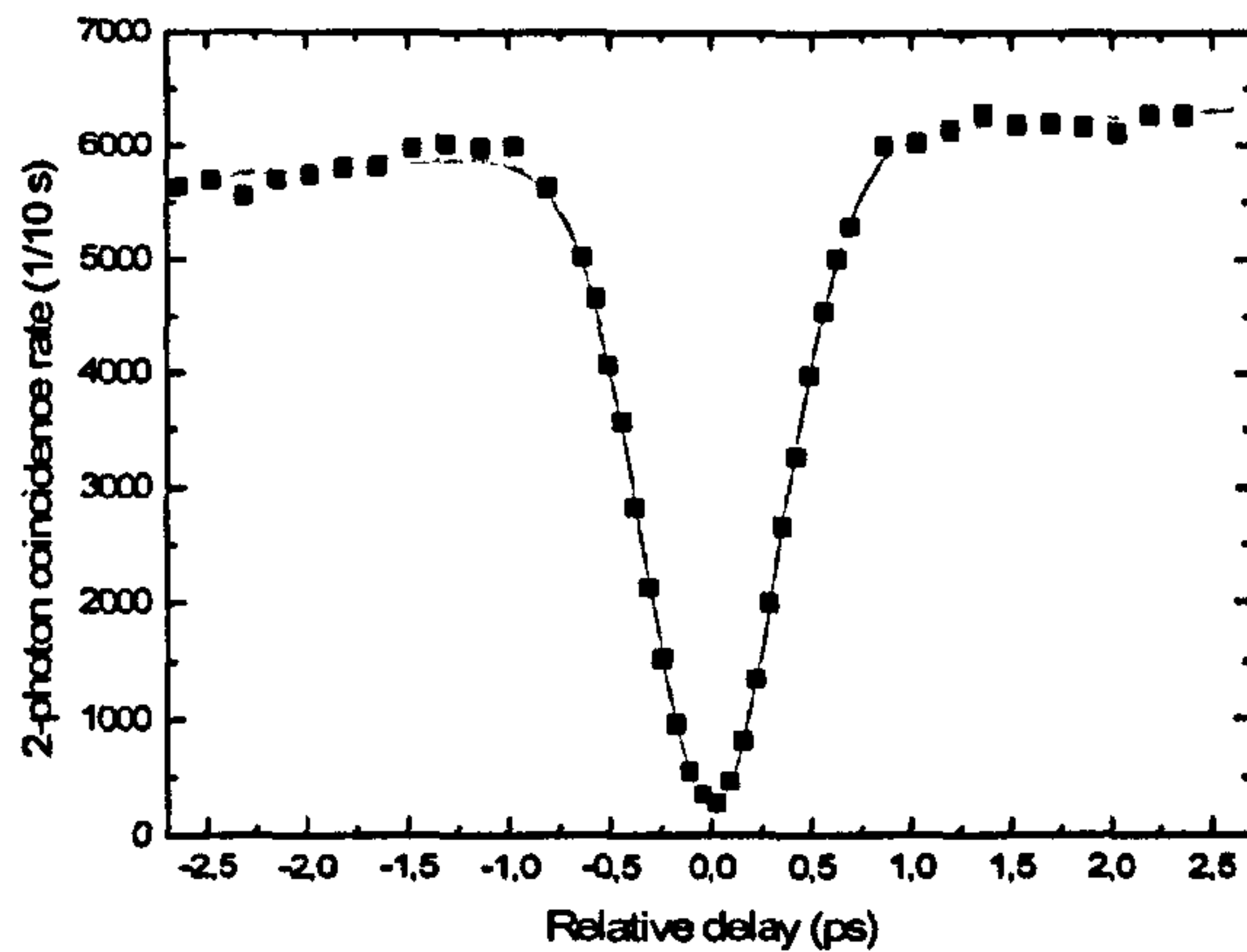
Figure 5.4: Quantum interference in a laser direct-write directional coupler. The number of coincident detections are shown as a function of the arrival delay between the two interfering photons. Error bars from Poissonian statistics are smaller than the point size and the fit is a Gaussian plus linear.
