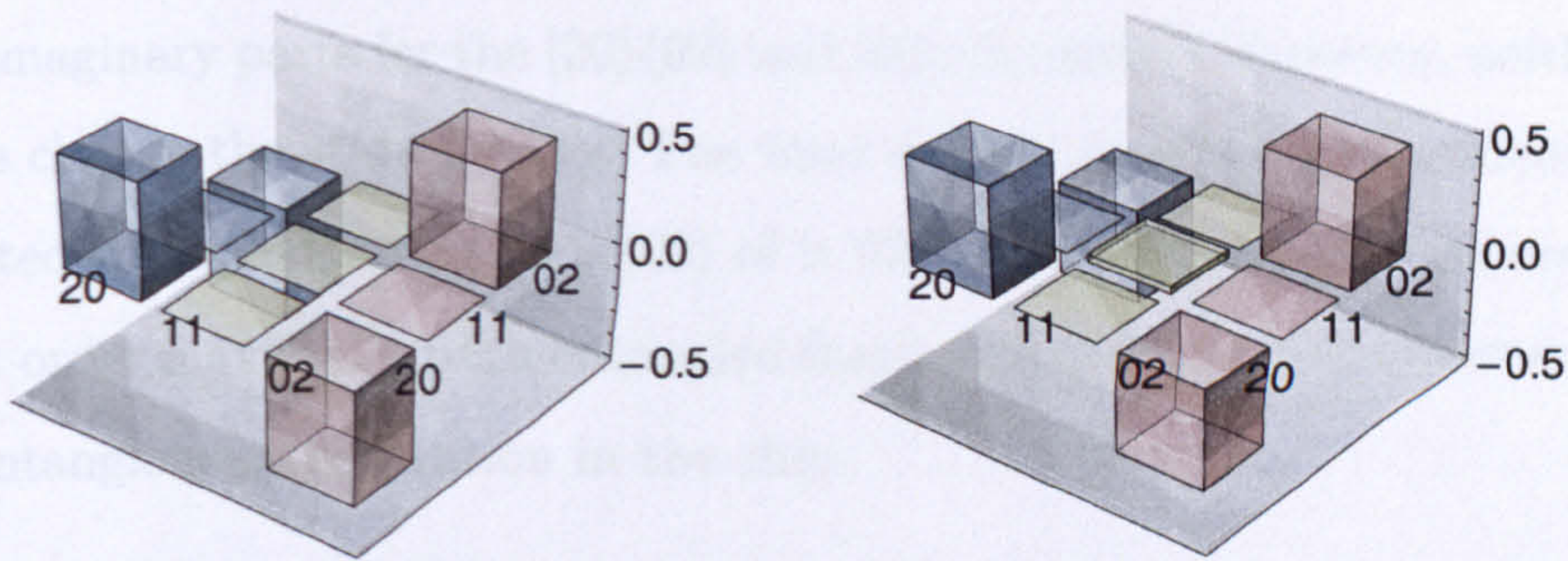
Figure 7.5: On-chip estimation of the density matrix for the entangled state |20\rangle - |02\rangle , ideal (left) and estimated (right).
