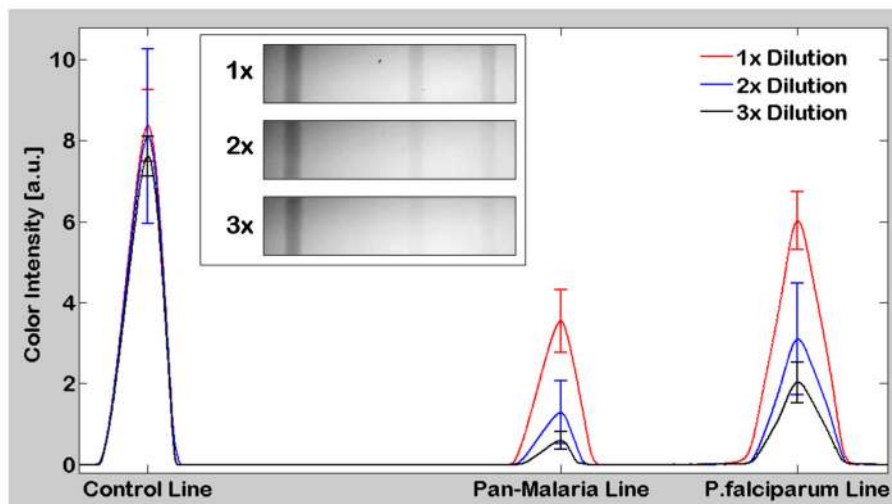
Fig. 6. Cross-sectional analysis of automatically processed malaria RDT images captured in reflection mode. The RDT reader shown in Fig. 1(a) was used to evaluate Malaria RDTs activated with 3 different batches of Positive Control Well Antigen (PCWA) at dilution levels of PCWA/20 \mu l (1x), PCWA/40 \mu l (2x), PCWA/60 \mu l (3x). The above figure illustrates the mean of 10 pre-processed RDT image cross-sections (for each dilution level) and the standard deviation of maximum peak values of each test line. Mean and standard deviation values of the Control, Pan-Malaria, and P. Falciparum lines of the 1x dilution level are 8.37, 3.54, 6.02; 0.89, 0.77, and 0.72, respectively. Mean and standard deviation values of the Control, Pan-Malaria, and P. Falciparum lines of the 2x dilution level are 8.11, 1.29, 3.10; 2.10, 0.77, and 1.38, respectively. Mean and standard deviation values of the Control, Pan-Malaria, and P. Falciparum lines of the 3x dilution level are 7.62, 0.60, 2.03; 0.50, 0.22, and 0.51, respectively. Exemplary cellphone images of RDTs for each dilution level are also shown in the inset.
