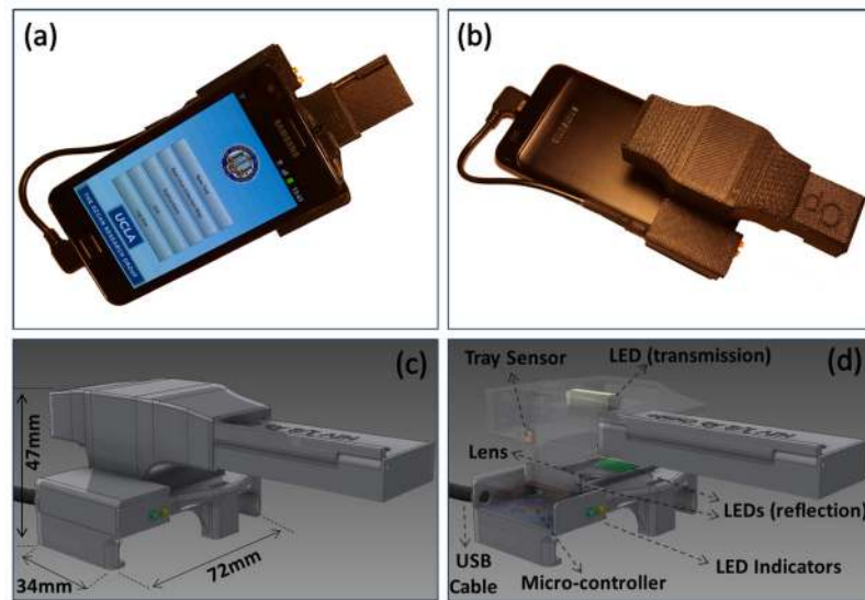
Fig. 7. A smart RDT reader prototype (attached to Samsung Galaxy S II) which is entirely powered by the cell-phone battery through a USB connection. Controlled through a cost-effective micro-controller, two LED indicators are also used in this design to automatically detect (i) if the attachment is successfully powered through USB; and (ii) if the RDT is properly loaded into the reader and is ready to be imaged.
