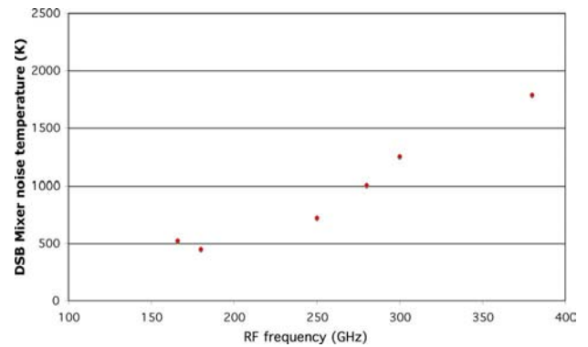
Fig. 6 A summary of mixer results using discrete diodes from RAL.
