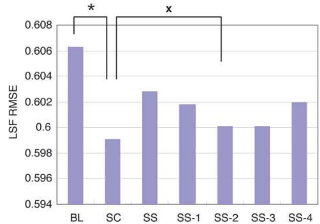
Fig. 9. Objective evaluation of LSF RMSE for State-Synchrony system with varying frame delay of articulatory features (“SS-1” to “SS-4”). The definition of each system can be found in Table I. “*” indicates the difference between two systems is significant and “x” indicates the difference is insignificant.
