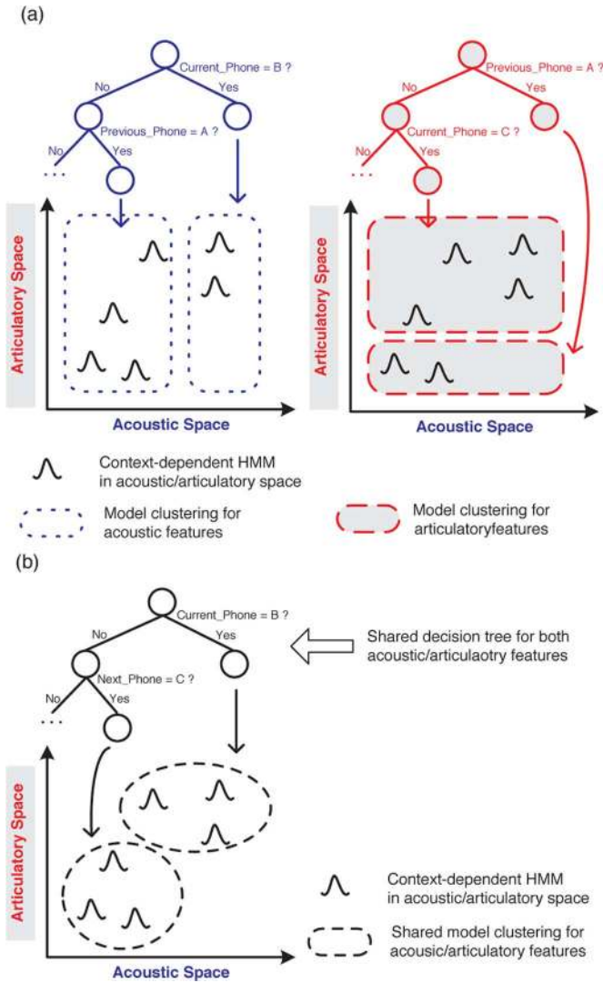
Fig. 3. Different model clustering approaches for combined acoustic and articulatory modeling. (a) Separate Clustering . (b) Shared Clustering .
