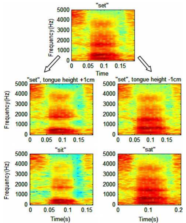
Fig. 19. Spectrograms of synthesized speech using the Feature-Dependency system with 100 transform classes (Top: word “set”; middle left: word “set,” with the z -coordinates of T1, T2, and T3 increased by 1 cm; middle right: word “set,” with the z -coordinates of T1, T2, and T3 decreased by 1 cm; bottom left: word “sit”; bottom right: word “sat”).
