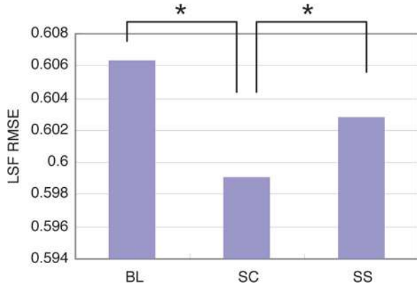
Fig. 8. Objective evaluation of LSF RMSE on Baseline (“BL”), Shared Clustering (“SC”), and State-Synchrony (“SS”) systems. The definition of each system can be found in Table I. “*” indicates the difference between two systems is significant.
