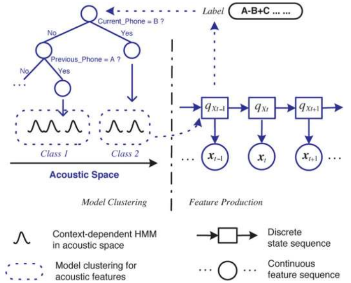
Fig. 2. Model structure of an HMM-based parametric speech synthesis system using only acoustic features.
