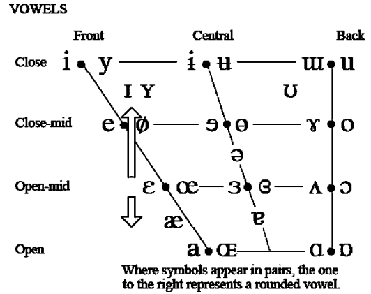
Fig. 16. IPA vowel chart. The arrows show the direction of vowel quality modification in our experiment.
