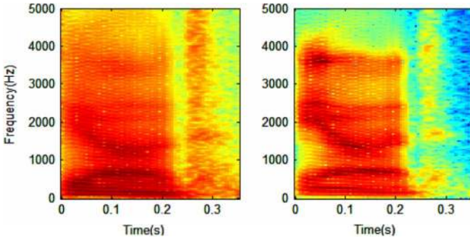
Fig. 15. Spectrograms for synthesized word “yard” using Feature-Dependency system without modification (left) and with a 1.5 scaling factor for the z -coordinates of all EMA receivers (right).
