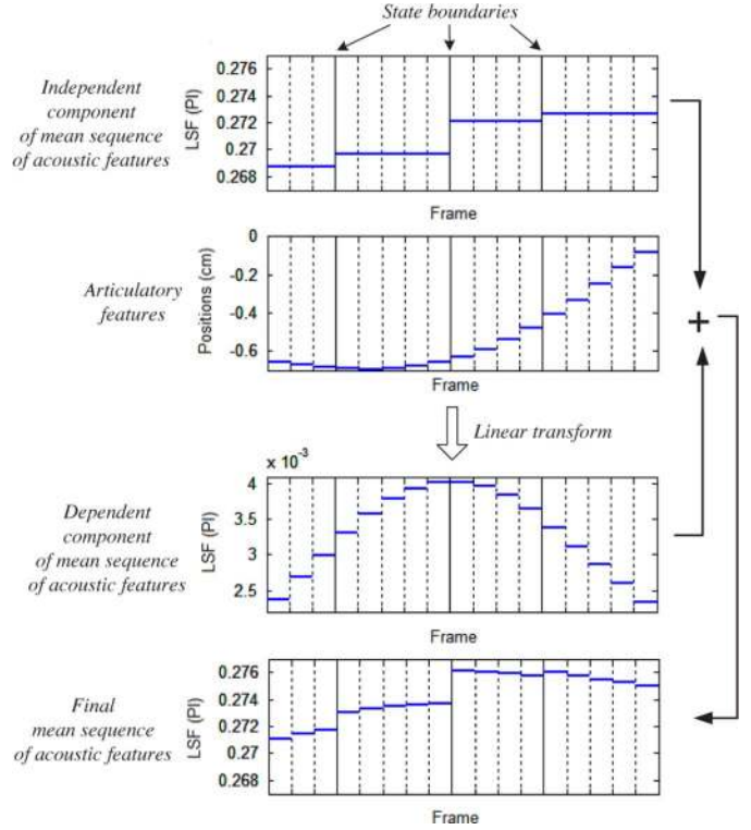
Fig. 5. Generation of HMM mean sequence of acoustic features in the Feature-Dependency system.
