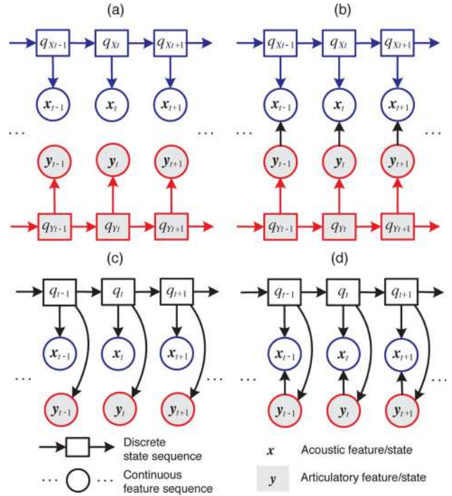
Fig. 4. Different feature production models for combined acoustic and articulatory modeling. (a) Asynchronous & Independent . (b) Asynchronous & Dependent . (c) Synchronous & Independent . (d) Synchronous & Dependent .
