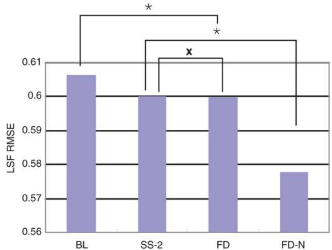
Fig. 10. Objective evaluation of LSF RMSE for Feature-Dependency system without natural EMA features in LSF generation (“FD”) and with natural EMA features in LSF generation (“FD-N”). The definition of each system can be found in Table I. “*” indicates the difference between two systems is significant and “x” indicates the difference is insignificant.
