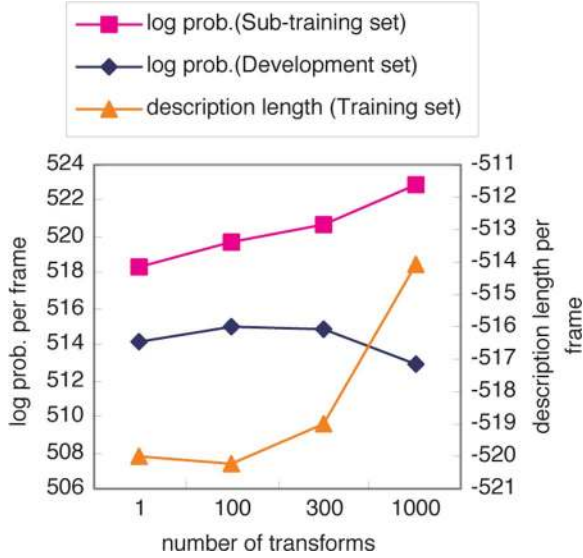
Fig. 7. Effect of varying the number of transforms in the Feature-Dependency system.
