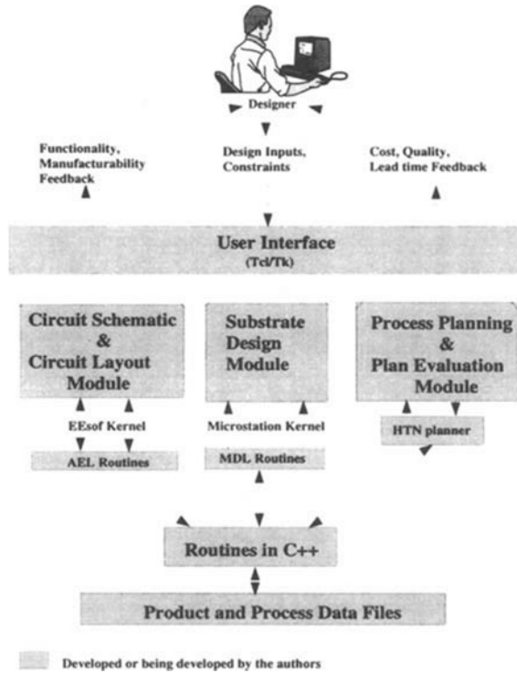
Figure 5 System architecture.
