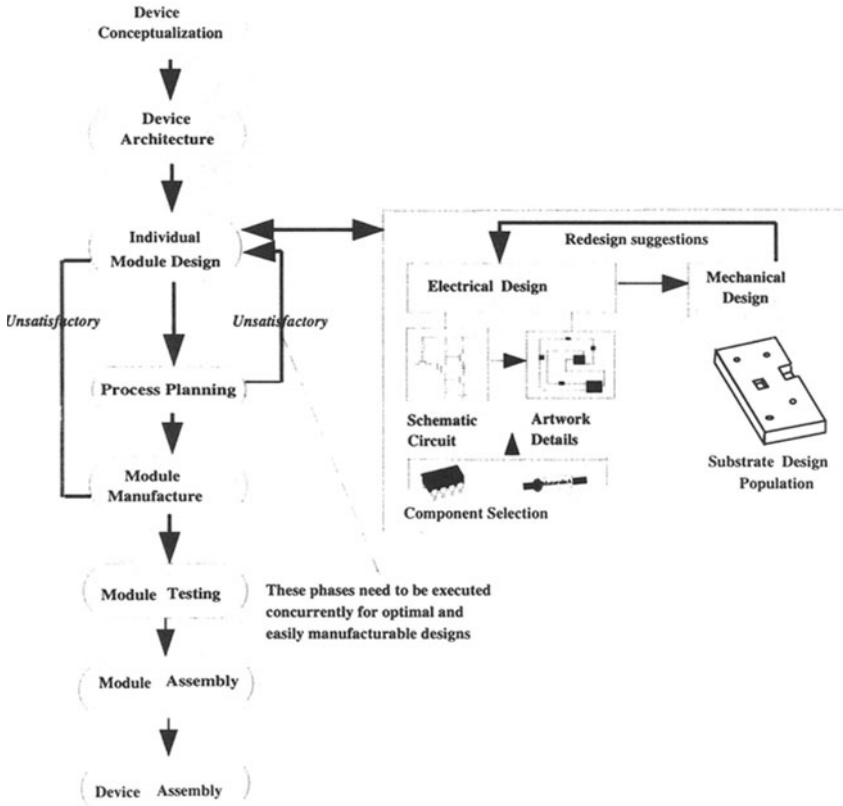
Figure 1 Design and manufacturing cycle for microwave T/R modules.
