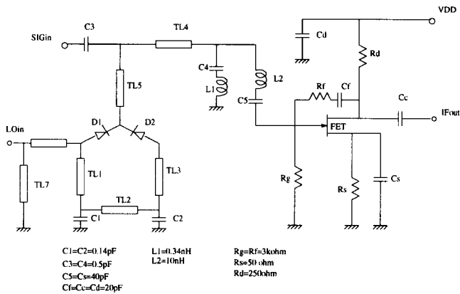
Figure 9 Mixer-IF amplifier schematic circuitry.
