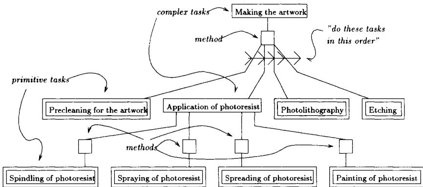
Figure 6 Part of the task network for microwave T/R module manufacture.
