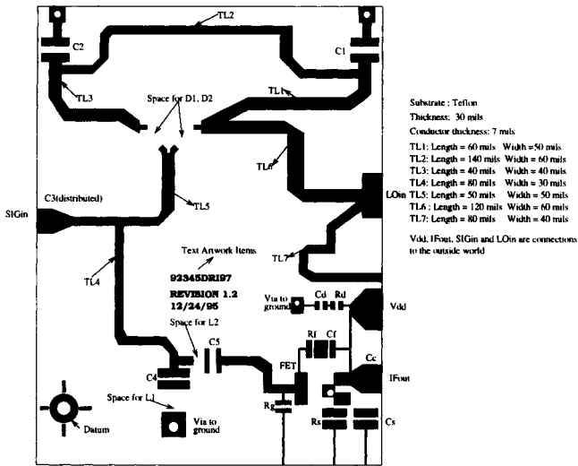
Figure 10 Mixer-IF amplifier circuitry layout.
