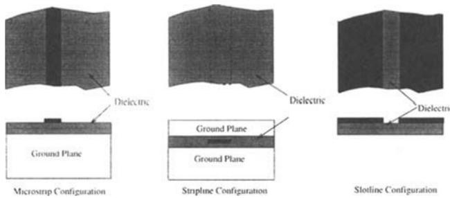
Figure 4 Transmission lines in microwave manufacturing.
