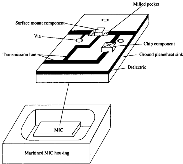
Figure 3 A typical microwave T/R module, consisting of the MIC substrate, and its housing.
