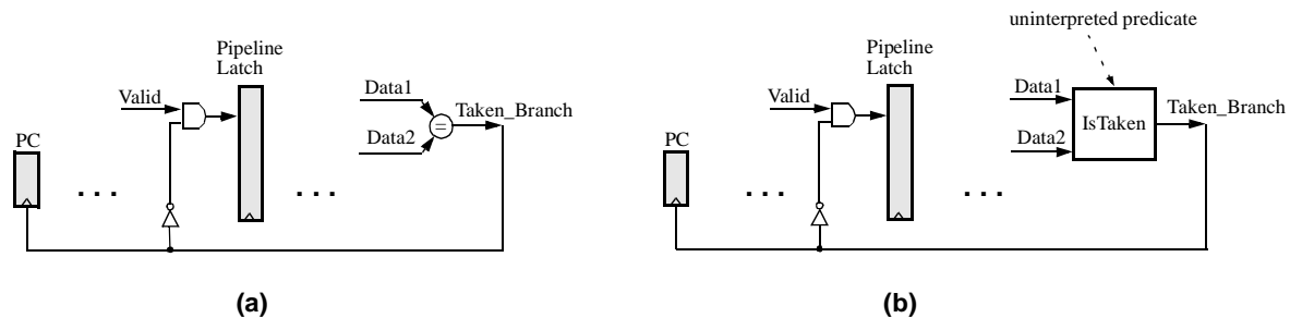
Figure 6. (a) The equality comparator that determines whether to take a branch-on-equal instruction, and driving signal Taken_Branch , appears in positive polarity when controlling the updates of the PC, but in negated polarity when controlling the squashing of subsequent instructions. (b) The equality comparator is abstracted with uninterpreted predicate IsTaken , thus avoiding negated equality between data operands Data1 and Data2 .
