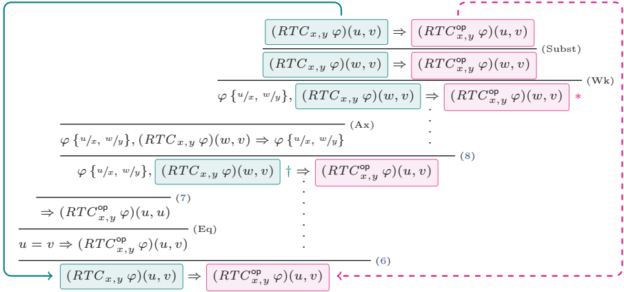
Fig. 2. Proof in RTcC_G^\omega of (RTC_{x,y} \varphi)(u, v) \Rightarrow (RTC_{x,y}^{op} \varphi)(u, v)
