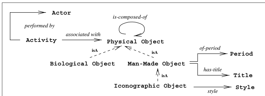
Fig. 3. A simple cultural ontology.
